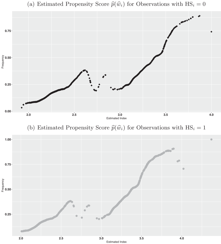
FIGURE A.4. Empirical distribution of \widehat{p}(\widehat{w}_i) with index restriction \widehat{w}_i = z_i'\widehat{\gamma} .
