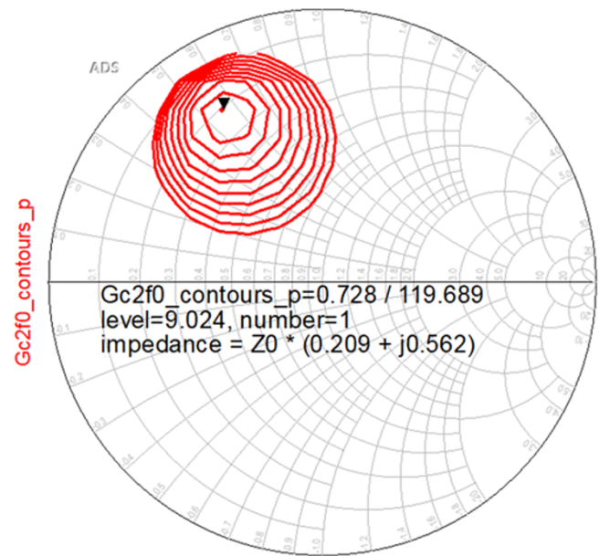
Figure 3. G_{c2f_0} simulated contours obtained at P_{in}=10 dBm with second harmonic LP, showing the impedance that maximizes G_{c2f_0} .
