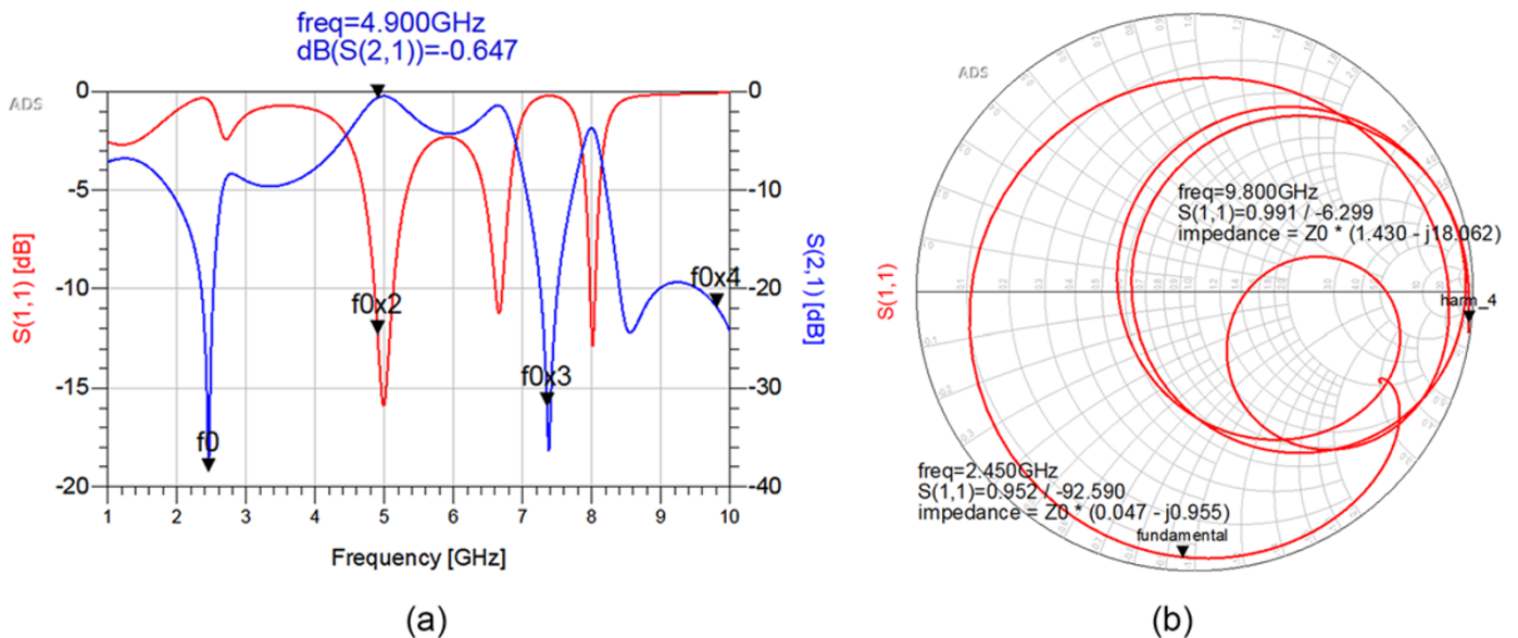
Figure 5. Simulated output matching network (a) S_{11} and S_{21} magnitude in dB. (b) S_{11} magnitude and phase.
