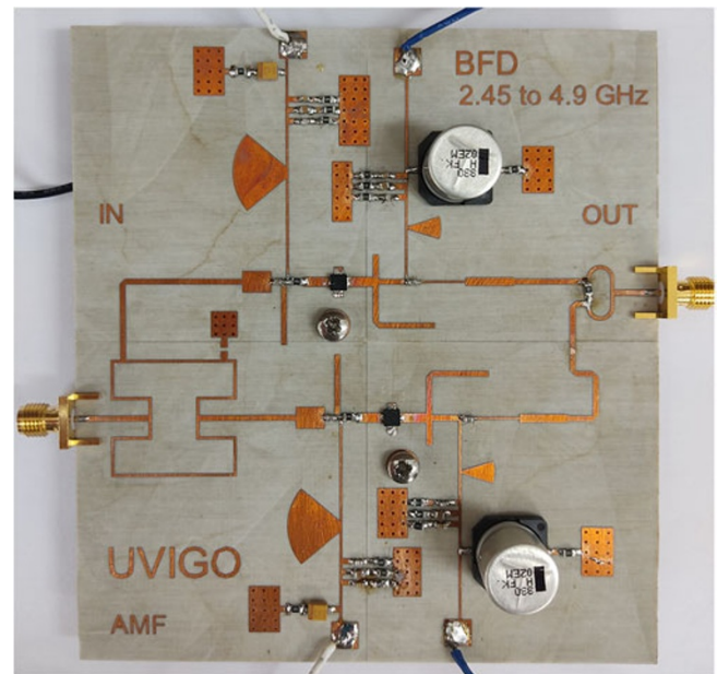
Figure 15. This work BFD prototype working at 2f_0 = 4.9 \text{ GHz} .
