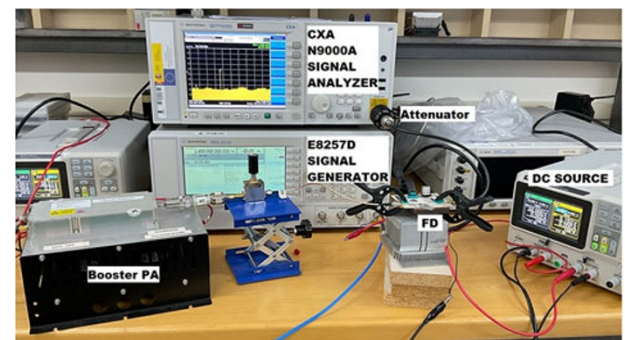
Figure 10. Measurement set-up used to perform large signal measurements.
