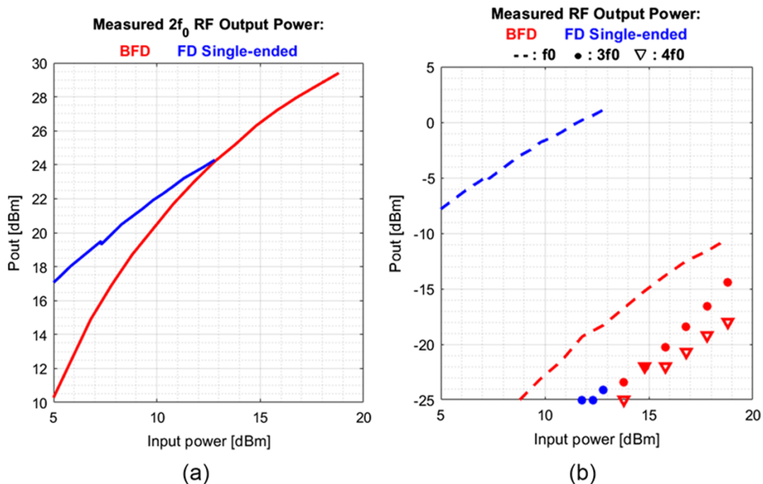
Figure 22. (a) Comparison of the measured P_{out2f_0} between the SE FD (blue) and the BFD (red) of this work. (b) Comparison of the measured P_{out} at other harmonics between the SE FD (blue) and the BFD (red) of this work.
