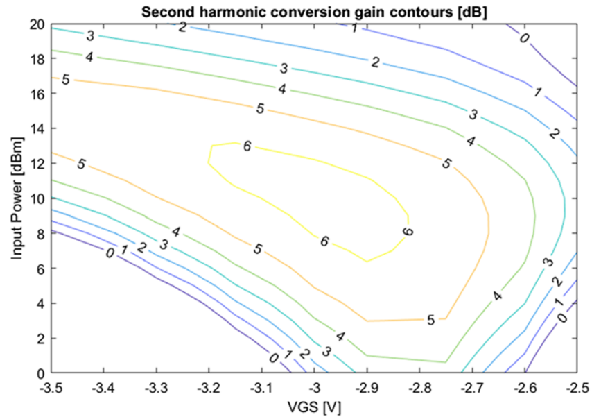
Figure 1. G_{c2f_0} simulated contours sweeping both P_{in} and V_{GS} .
