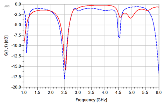
Figure 9. Measured (blue dashed line) and simulated (red continuous line) SE FD prototype S_{11} .
