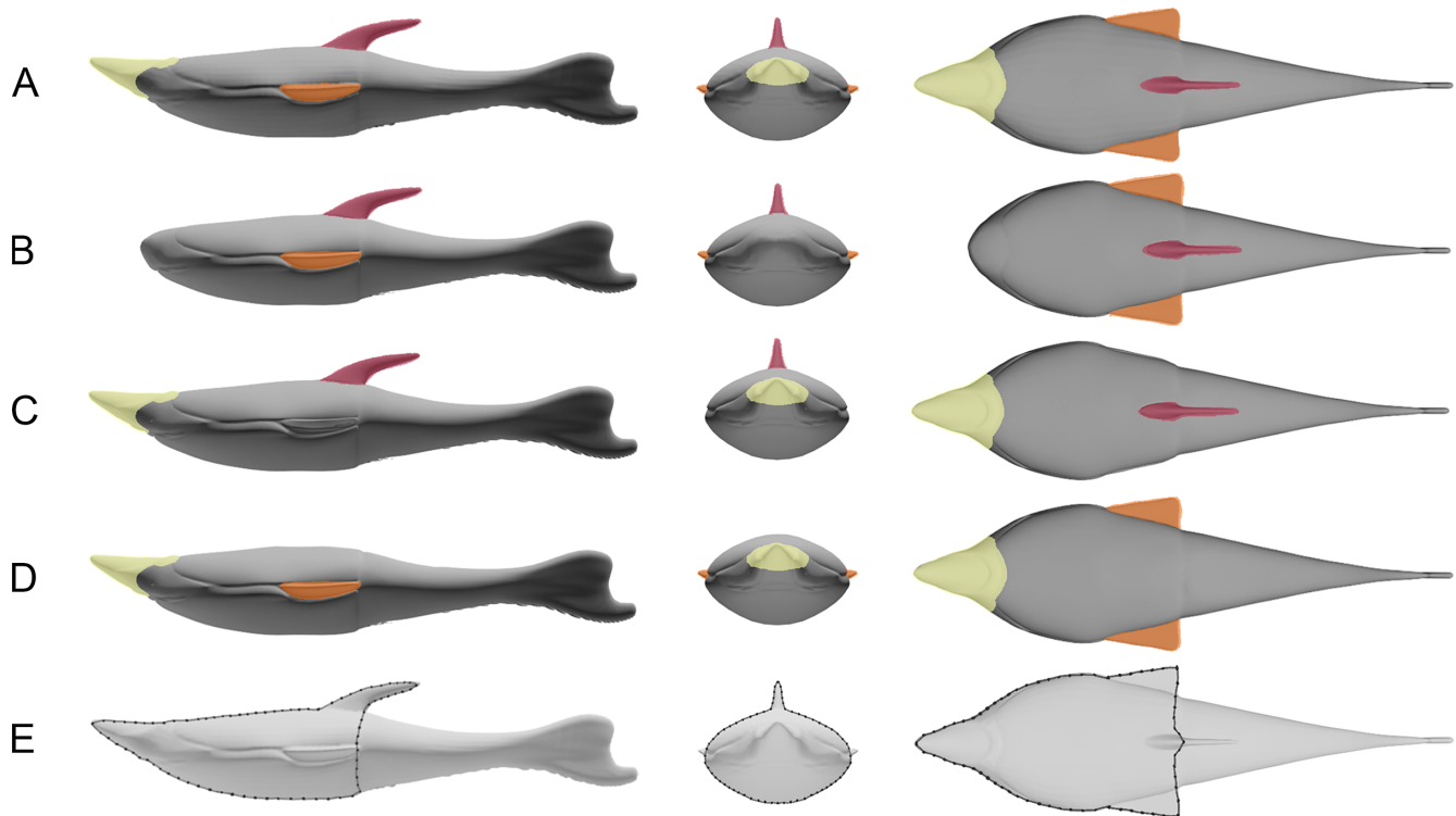
Figure 1. Preprocessing of 3D models and landmark configurations. A , Visualization of the 3D model showcasing frontal, dorsal, and lateral headshield processes, highlighted in yellow, red, and orange, respectively. The original 3D models underwent preprocessing steps before computational fluid dynamics (CFD) simulations involving the removal of (B) frontal, (C) lateral, and (D) dorsal headshield processes. E , The landmark configurations utilized in the geometric morphometric analyses are depicted. As an illustrative example of a pteraspidomorph, the 3D model of Errivaspis waynensis is presented in lateral, frontal, and dorsal views, arranged from left to right.
