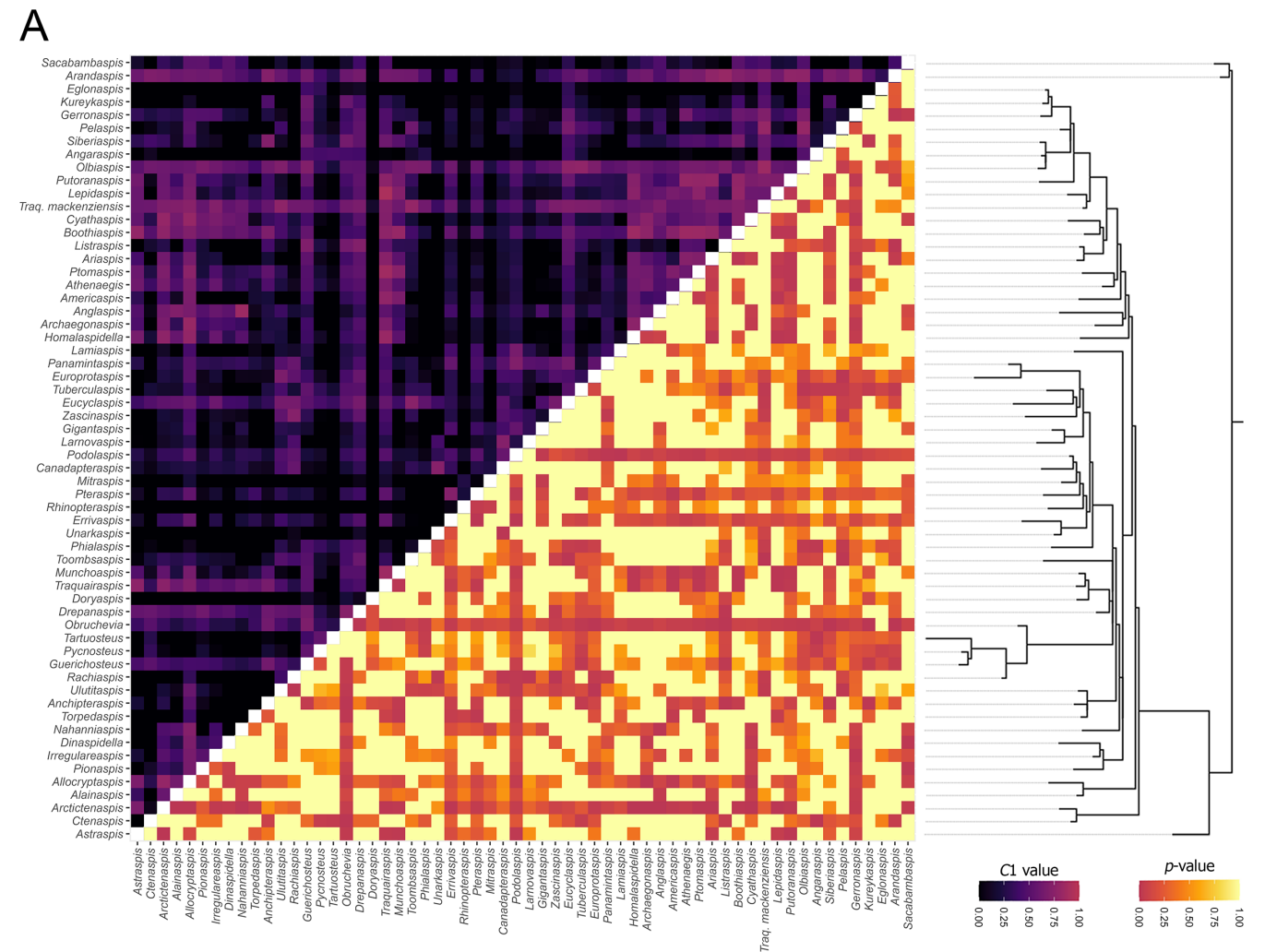
Figure 5. Quantifying convergence in headshield processes of Pteraspidomorphi through Stayton's (A) C1 and (B) C1 metrics. The Stayton's C1 and C1 metrics, depicted in purple, provide a measure of convergence strength, while the accompanying p -values, shown in yellow-orange, indicate the statistical significance of the observed convergence. Note that instances where C1 metrics and p -values are displayed in white result from uninformative analyses, typically due to comparisons between sister taxa or taxa lacking contemporaneous ancestral nodes. The phylogenetic tree is based on Randle et al. (2022), Glinskiy (2018), Dec (2019b), and Janvier (1996).
