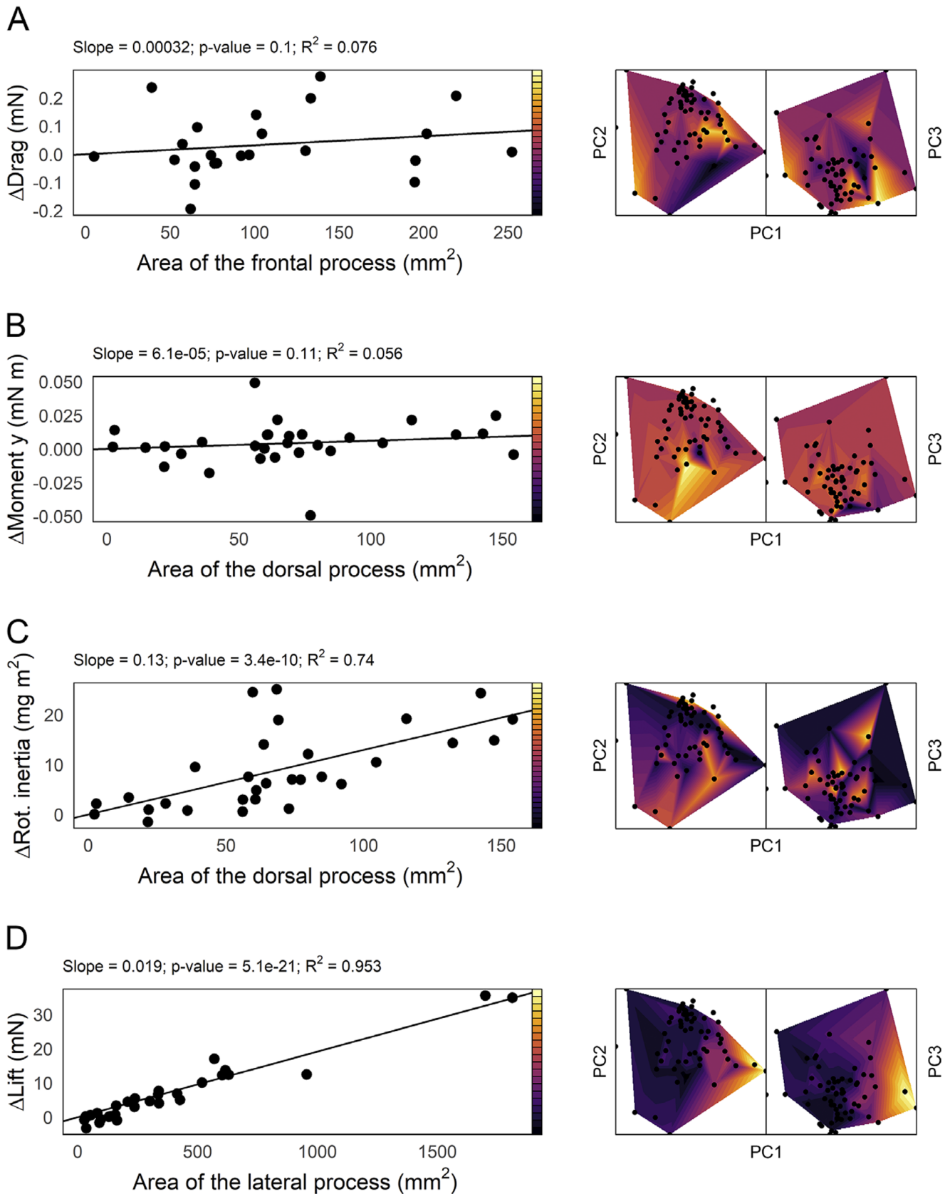
Figure 6. Hydrodynamic impact of headshield processes of Pteraspideromorphi. Differences in various biomechanical parameters between the unaltered original models and those with specific processes removed are depicted through linear regression plots against the corresponding process area (depicted on the left), while complementary heat maps are overlaid onto the morphospaces (illustrated on the right). Impact of the frontal process on (A) the difference in drag; impact of dorsal process on the difference in (B) yawing moment and (C) rotational inertia; and impact of the lateral processes on the difference in (D) lift, (E) lift-to-drag ratio, (F) rotational inertia, (G) yawing moment, and (H) pitching moment. Negative values for \Delta M_{\text{pitch}} and \Delta M_{\text{yaw}} indicate a stabilizing effect, while positive values indicate a destabilizing effect.
