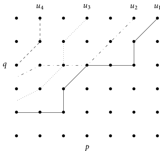
Figure 3: (\bar{P}_1, \bar{P}_2, P_3, \dots, P_r) .
