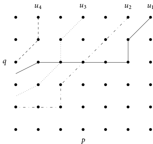
Figure 2: (P_1, \dots, P_r) .
