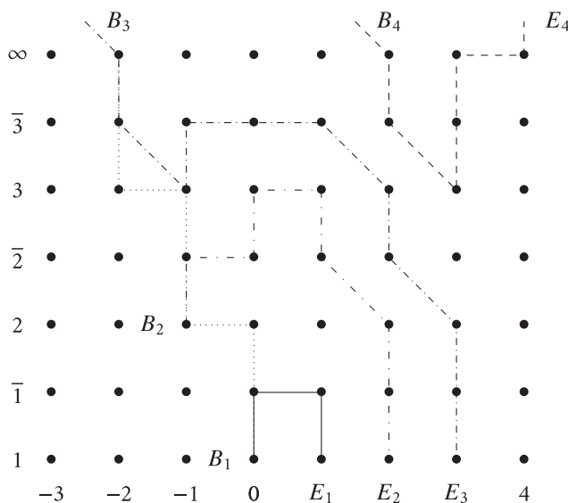
Figure 7: (P_1, P_2, P_3, P_4) satisfying the condition in Example 8.2.
