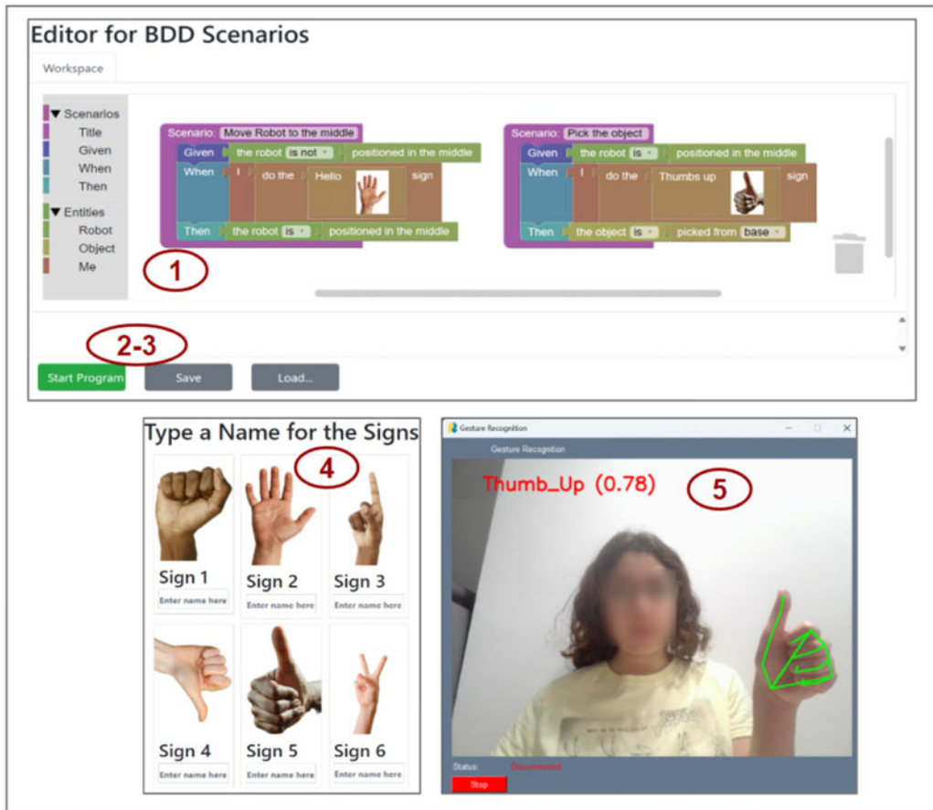
Figure 3. Interface elements of the development environment.
