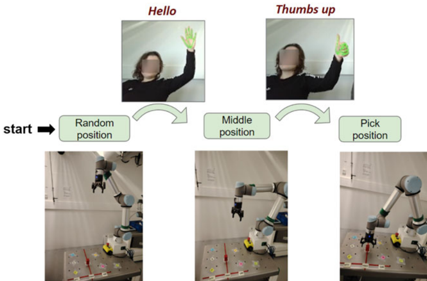
Figure 1. State diagram from sample sequence in Listing 2. User gestures trigger robot state transitions.
