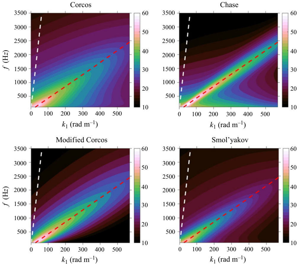
Figure 19. Wavenumber–frequency spectrum estimates from various models for the array of sensors.
