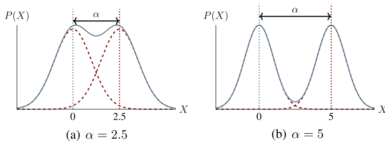
Figure 1. Illustrative example for Y \rightarrow X .
