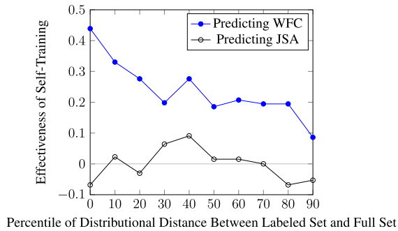
Figure 2. Relationship between effectiveness of self-training and representativeness of labeled set. Note: WFC, work-family conflict; JSA, job satisfaction. Source: Swiss Household Panel (SHP).
