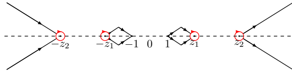
Figure 14. The jump contour \Sigma^E for the E(z; \xi, c) . The red circles are \partial U .
