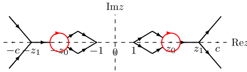
Figure 9. The jump contour \Sigma^E for the E(z) . The red circles are \partial U .
