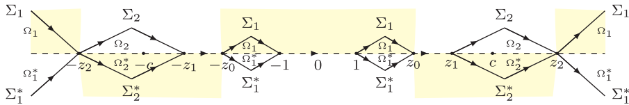
Figure 10. The domains \Omega_j and curves \Sigma_j , j = 1, 2 . The yellow region means \text{Im}[g](z) < 0 while white region means \text{Im}[g](z) > 0 .
