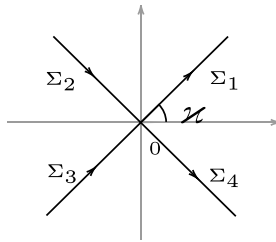
Figure 15. Orient of \Sigma_k, k = 1, 2, 3, 4 .
