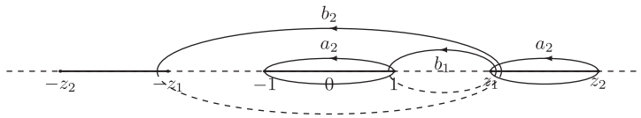
Figure 12. The canonical homology basis \{a_j, b_j\}_{j=1}^2 of the genus 2 Riemann surface.
