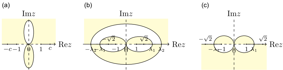
Figure 2. In the white region, \text{Im}[p^{(-)}] > 0 , while in another region, \text{Im}[p^{(-)}] < 0 . (a) \xi < 3/4 ; (b) 3/4 < \xi < 1 ; (c) 1 \leq \xi < 3 .
