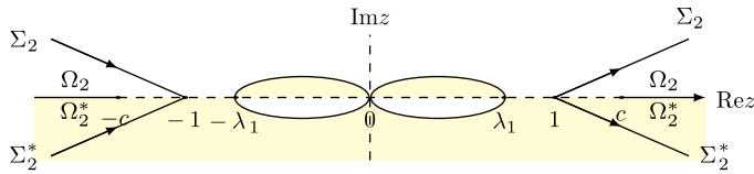
Figure 6. The region \Omega_2 \cup \Omega_2^* and curve \Sigma_2 \cup \Sigma_2^* . In this case \{(\xi, c) : \xi > 1 + 2/c\} , \text{Im}[\theta^{(+)}](z) < 0 in yellow region while \text{Im}[\theta^{(+)}](z) > 0 in white region. And critical line \text{Im}[\theta^{(+)}](z) = 0 is black solid line.
