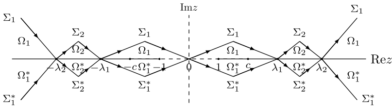
Figure 4. Figure of curves \Sigma_j and domains \Omega_j , j = 1, 2 , in the case of \{(\xi, c) : 1 < c \leq \lambda_1, 3/4 < \xi < 1\} .
