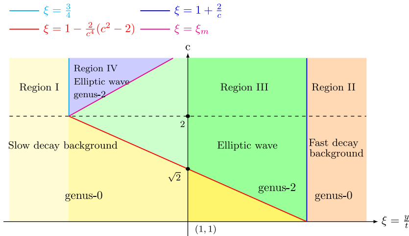
Figure 1. Asymptotic approximations of the mCH equation in different space-time- (\xi, c) regions, where the Regions I ( yellow ) and II ( orange ) corresponding to genus-0, they are slow-decay and fast-decay background regions, respectively; The Regions III ( green ) and IV ( purple ) corresponding to genus-2 region, they are the first-type and second-type elliptic wave regions. Here, \xi_m is the critical condition that under the case of Region III, the stationary point of g -function merges to c . The Region I is a unit of three subregions. We use three shades of yellow to distinguish these three subregions. The Region III is a unit of two subregions, where we use two shades of green to distinguish it.
