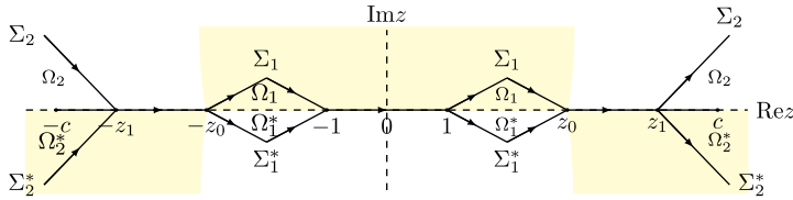
Figure 8. The opened jump contours \Sigma^{(1)} and opened domains \Omega_j \cup \Omega_j^* , j = 1, 2 . The yellow region means \text{Im}[g] < 0 , while white region means \text{Im}[g] > 0 .
