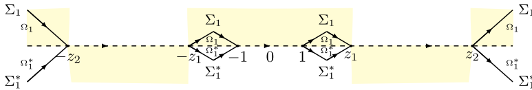
Figure 13. The region of \Omega_1 \cup \Omega_1^* and the contour \Sigma_1 \cup \Sigma_1^* . The shaded region means \text{Im}[g](z) < 0 , while white region means \text{Im}[g](z) > 0 .
