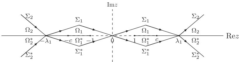
Figure 5. Figure of curves \Sigma_j and domains \Omega_j , j = 1, 2 , in the case of \{(\xi, c) : 1 < c \leq \lambda_1, 1 \leq \xi < 3\} .
