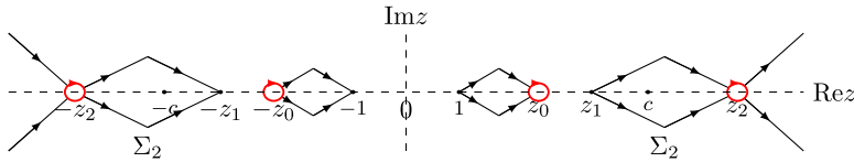
Figure 11. The jump contour \Sigma^E for the E(z) . The red circles are \partial U .
