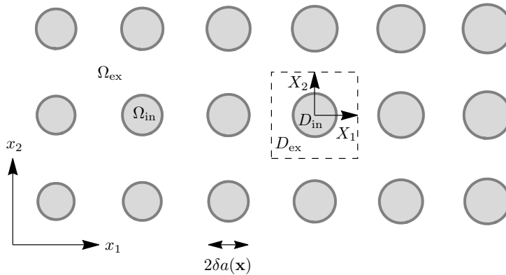
Figure 1. An example of a 2D composite. Perfectly dielectric inclusions shown in grey lie on a periodic array within an insulator. The inclusions have a radius a(\mathbf{x}) which varies slowly across the domain. In this example a(\mathbf{x}) = 0.3 + 0.1(x_1 + x_2) so that the boundaries of the inclusions are |(x_1, x_2) - \delta(n, m)| = \delta(0.3 + 0.1x_1 + 0.1x_2) , for n, m \in \mathbb{Z} .
