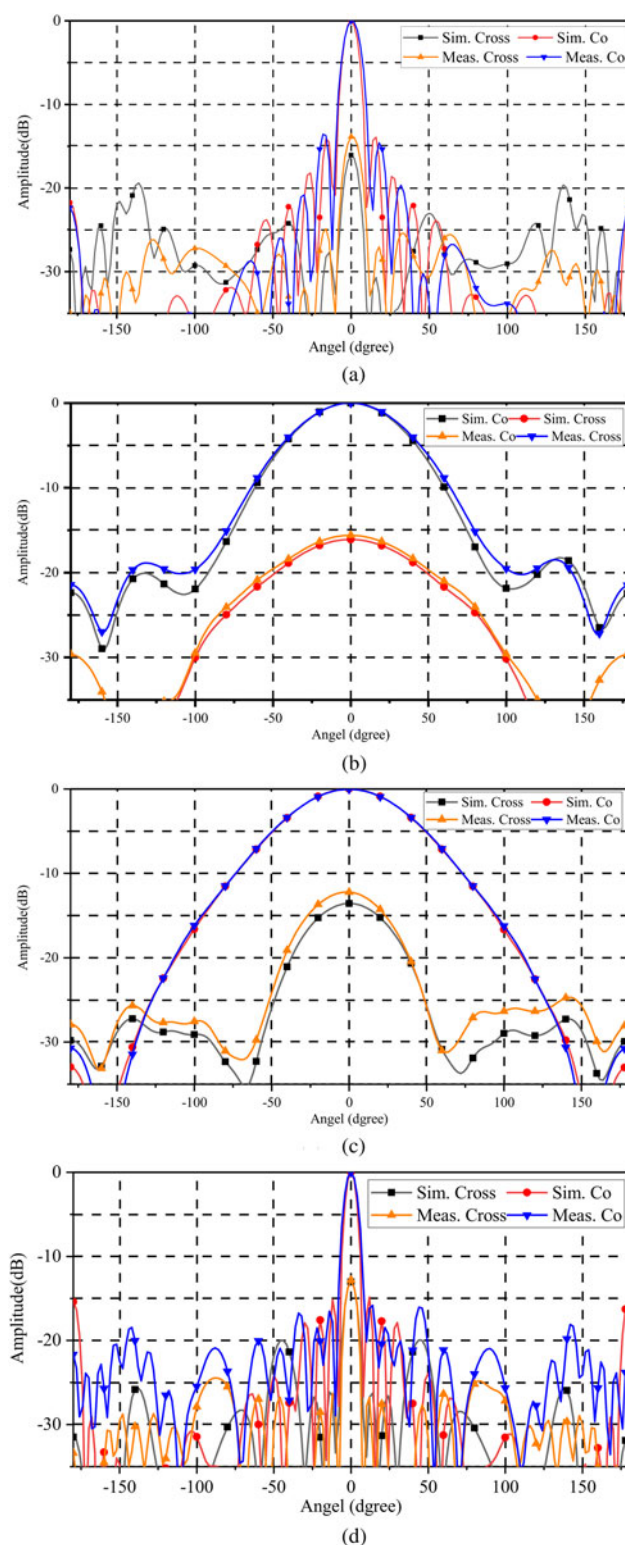
Fig. 15. Measured and simulated normalized radiation patterns of VP array and HP array: (a) yoz -plane at 9.6 GHz, (b) xoz -plane at 9.6 GHz, (c) xoz -plane at 12 GHz, and (d) yoz -plane at 12 GHz.
