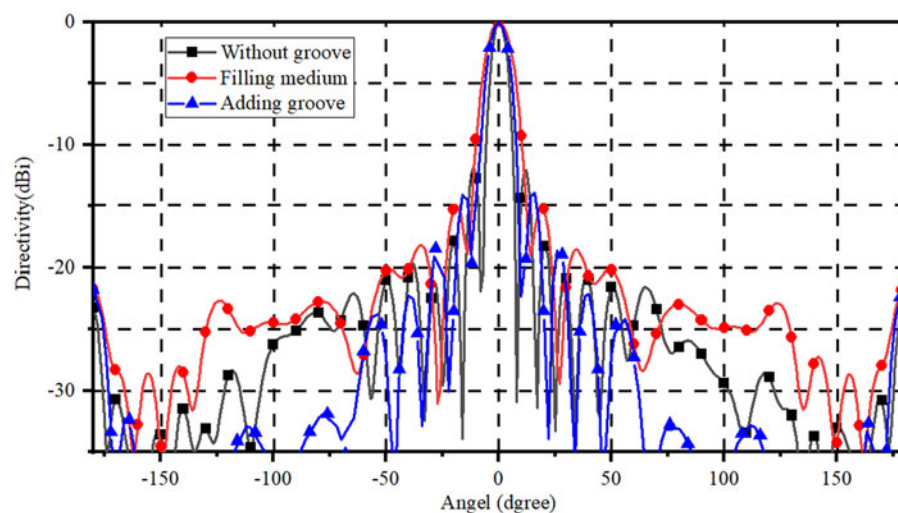
Fig. 7. Patterns of three antenna array.
