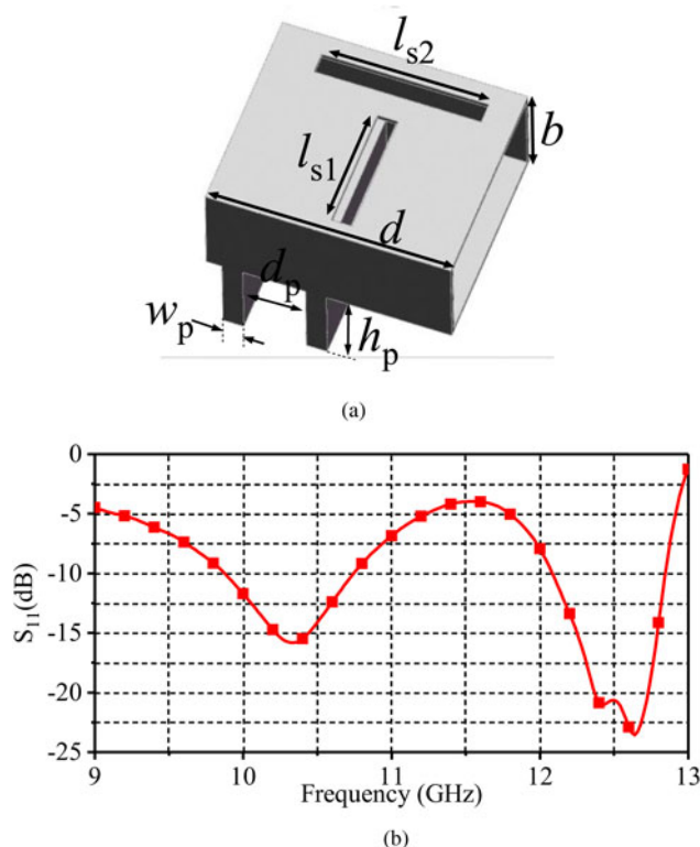
Fig. 8. (a) Model with two grooves at the bottom and (b) the S_{11} of the model.
