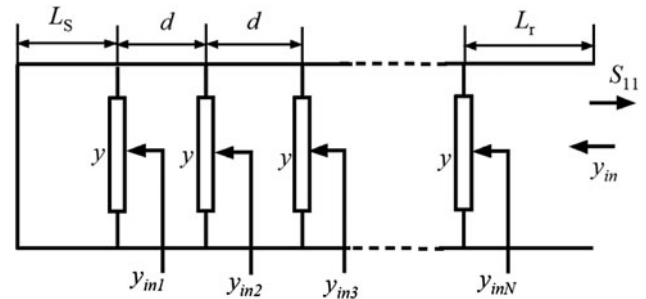
Fig. 3. Equivalent transmission line model of N -element slotted uniform linear array terminated in a short circuit.
