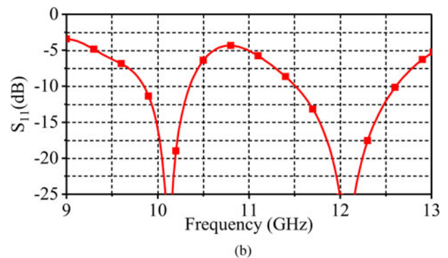
Fig. 4. Simulated dual-band unit of S_{11} .
