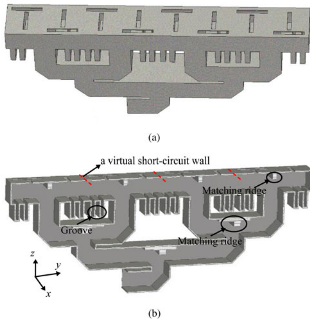
Fig. 1. Model of the antenna: (a) overview of the antenna and (b) sectional view of the antenna.
