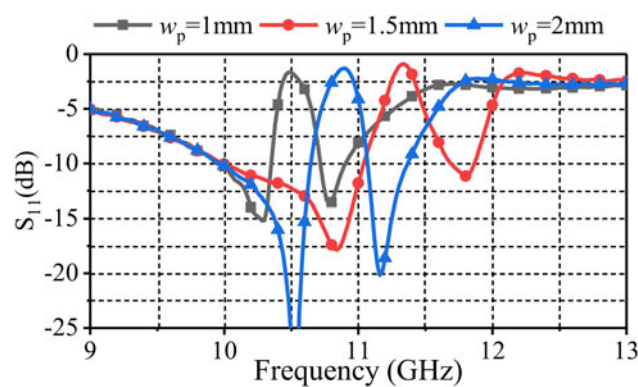
Fig. 11. Parametric analysis of the w_p of S_{11} .
