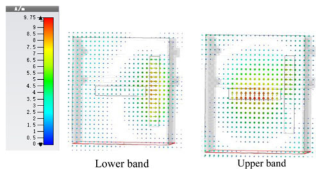
Fig. 5. Simulated surface current distribution of the unit.
