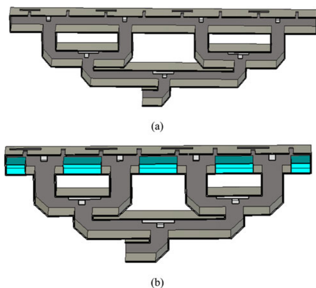
Fig. 6. (a) Without groove antenna array and (b) dielectric-added and non-grooved antenna array.
