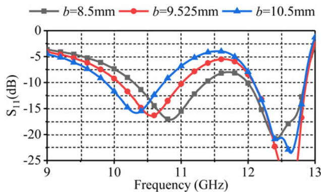
Fig. 9. Parametric analysis of the b of S_{11} .
