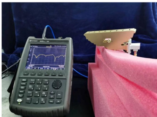
Fig. 13. Fabricated antenna.
