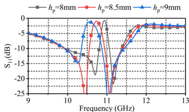
Fig. 12. Parametric analysis of the h_p of S_{11} .
