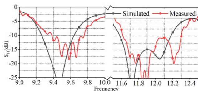
Fig. 14. Simulated and measured S_{11} .
