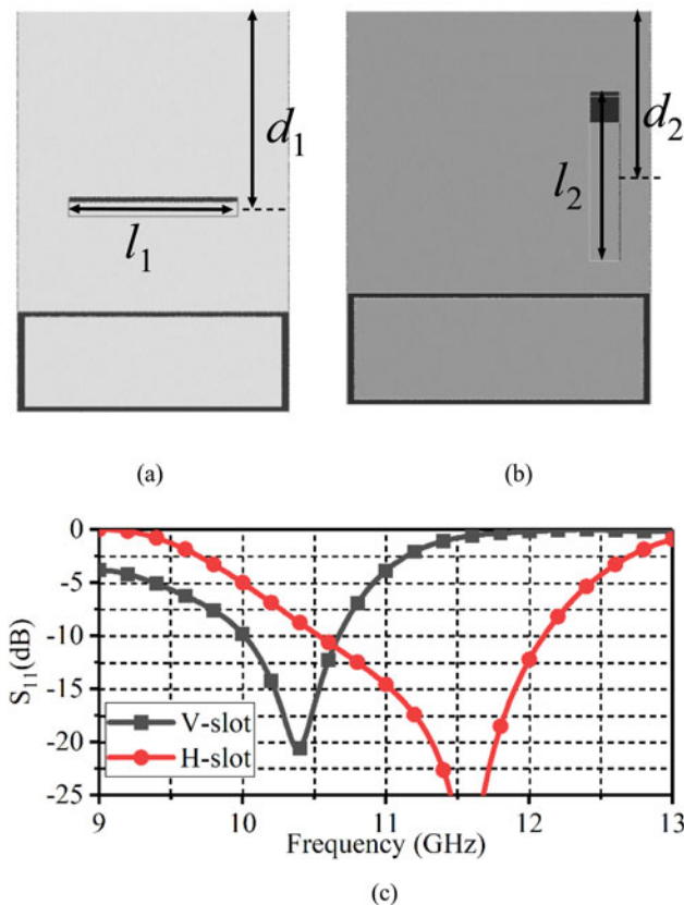
Fig. 2. (a) Model of horizontal polarization antenna; (b) the model of vertical polarization antenna; and (c) the simulated S_{11} ( l_1 = 12 mm, l_2 = 15 mm).
