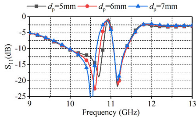
Fig. 10. Parametric analysis of the d_p of S_{11} .
