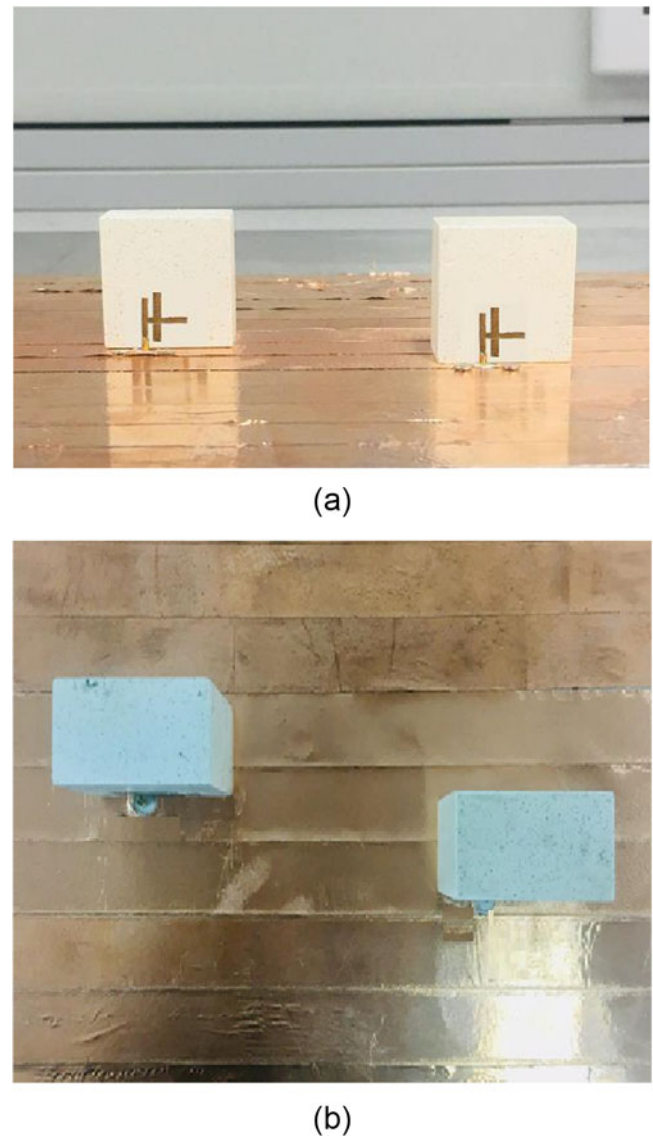
Figure 5. Photograph of the proposed CP MIMO DRA. (a) Front view. (b) Top view
