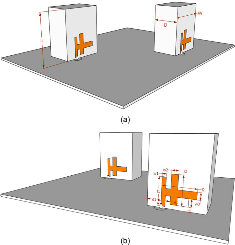
Figure 1. (a) Proposed circularly polarized multiple-input-multiple-output DRA. (b) Optimized design configuration.
