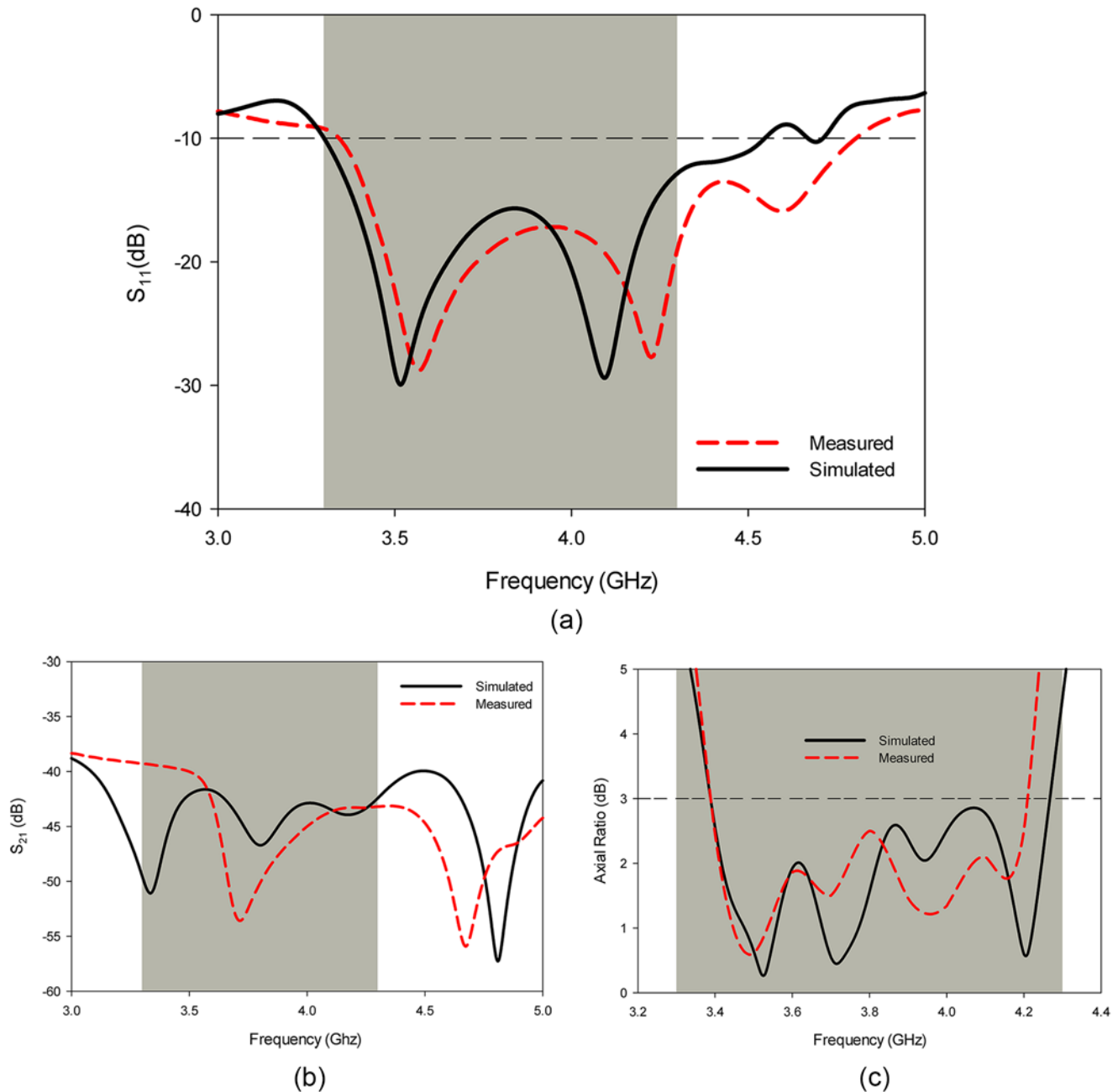
Figure 6. Measured and simulated results of the proposed CP MIMO DRA. (a) S_{11} , (b) S_{21} , and (c) axial ratio.
