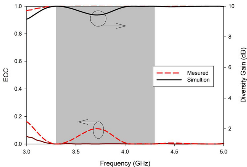
Figure 8. ECC and DG of the CP MIMO antenna.
