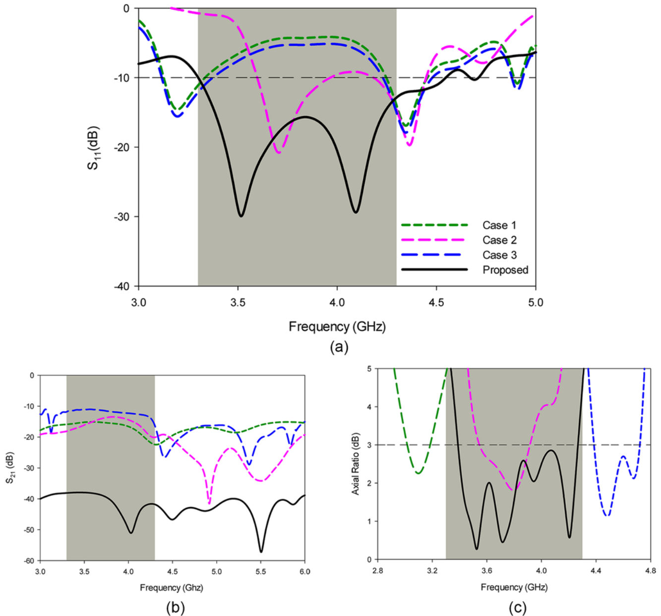
Figure 3. Case study of the proposed CP MIMO DRA. (a) S_{11} , (b) S_{21} , and (c) axial ratio.
