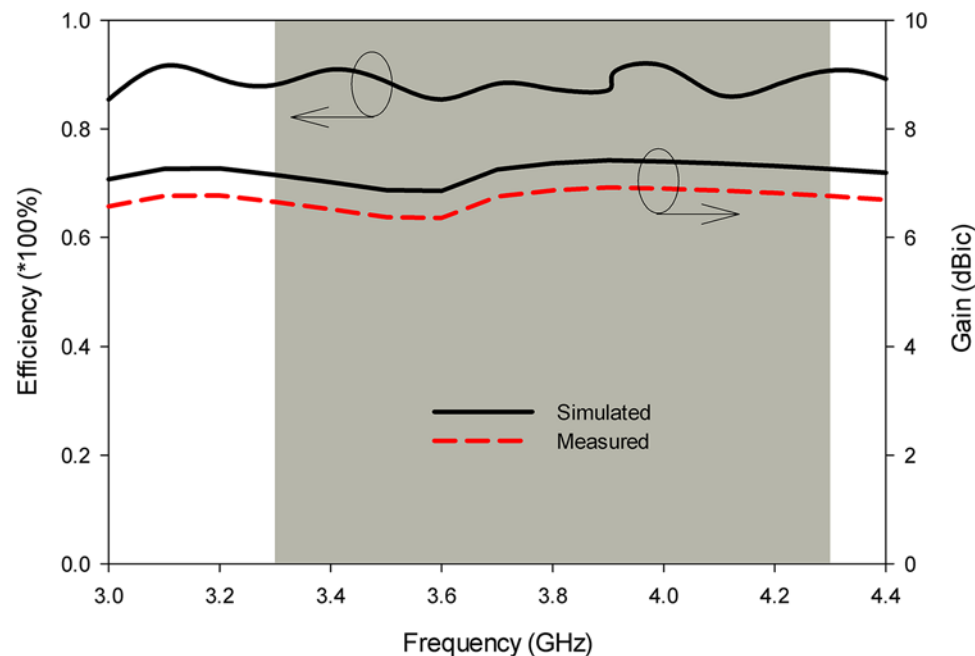
Figure 9. Efficiency and gain of the CP MIMO antenna.
