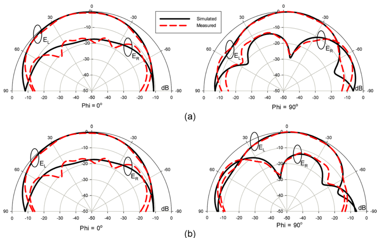
Figure 7. Radiation patterns of the proposed CP MIMO DRA at 3.5 GHz. (a) Port 1. (b) Port 2.
