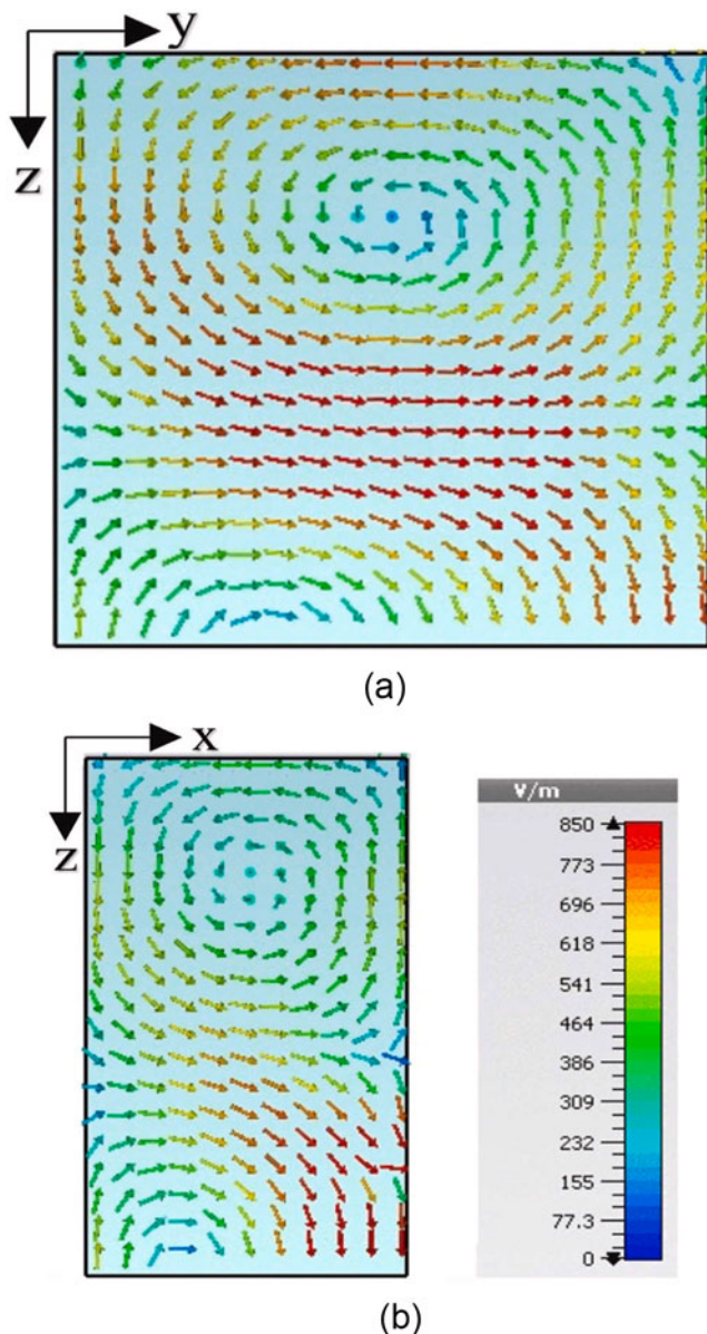
Figure 4. E-field distribution on each DRA. (a) TE_{\delta 13}^x at 3.49 GHz. (b) TE_{1\delta 3}^y at 4.15 GHz.
