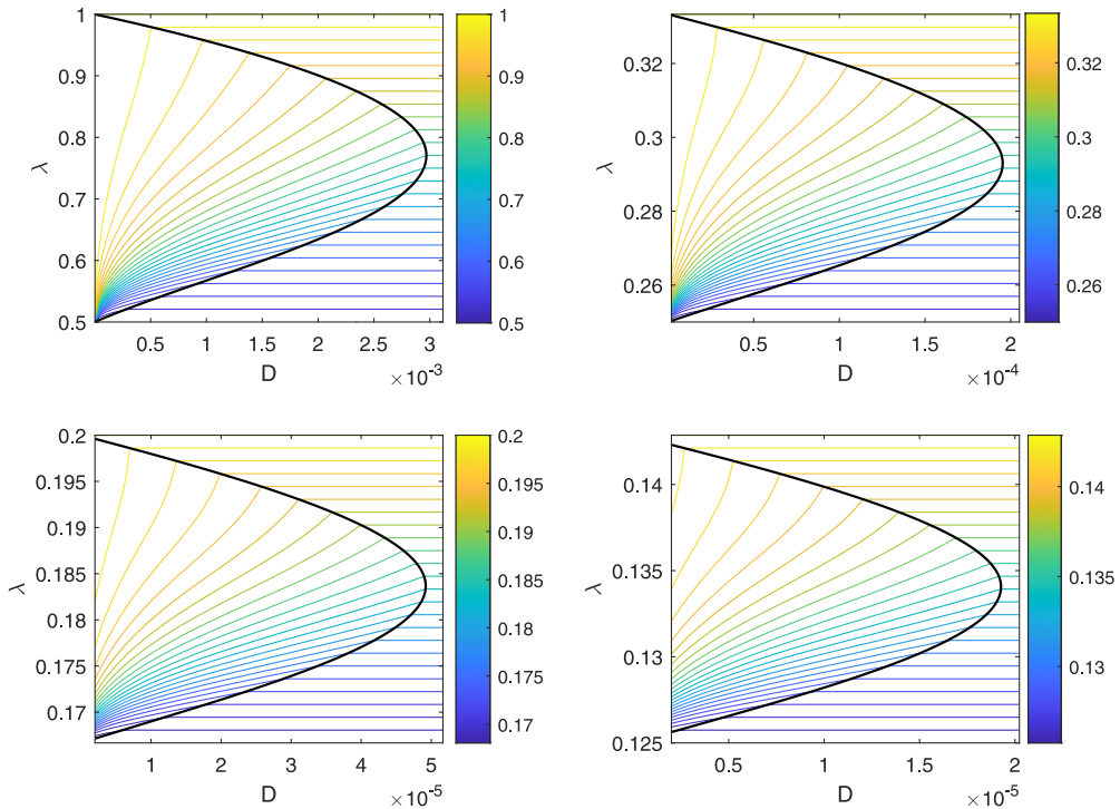
Figure 2. The L^1 norm, A(\lambda, D) , of the nontrivial, non-negative, periodic steady states identified in (NBI). The first four tongue regions are shown in the (D, \lambda) plane.
