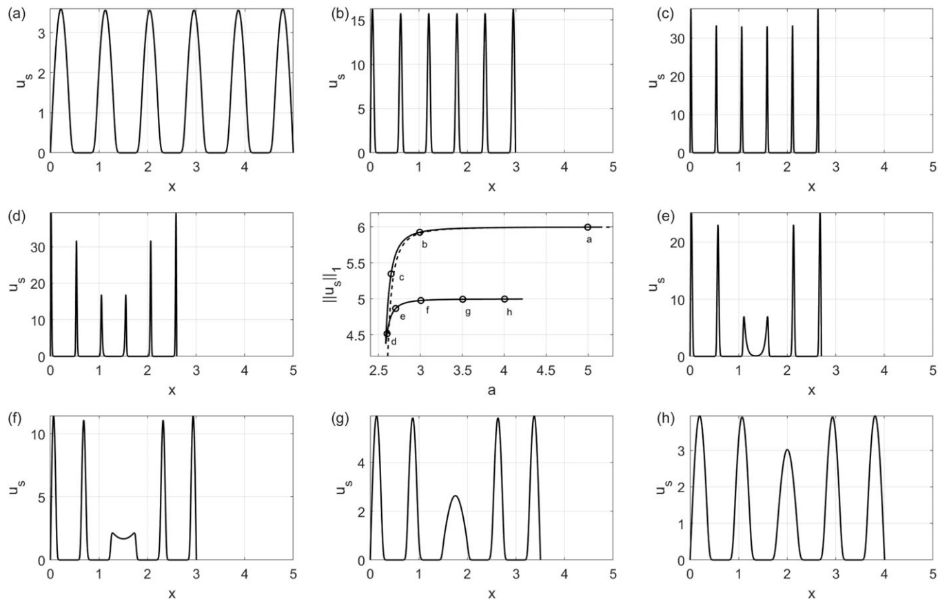
Figure 5. The profile of the steady state u_s as the r=6 to r=5 echelon of the bifurcation diagram is traversed. The central panel shows the relevant portion of the bifurcation diagram, with the broken line given by (80). Note the different u_s -axis limits in the other panels, individually labelled (a) to (h), and identified on the central panel. The most dramatic changes in functional form occur along the upper branch of the bifurcation curve, where the peaks become taller and thinner, and then at the left-hand side of the bifurcation curve, where the number of peaks changes by one. Note that only solutions (a) to (c) are stable.
