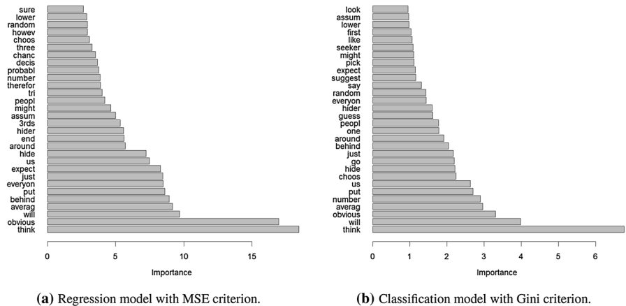
Fig. 4 Variable importance in the BCHS dataset
