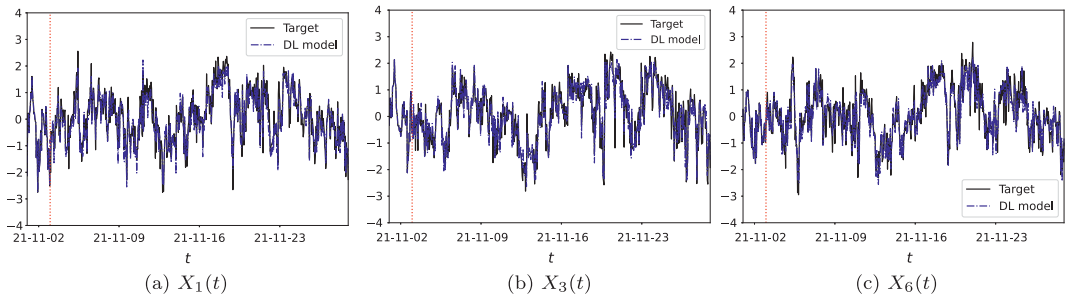
Figure 12. Target versus synthetic time series produced by the deep learning model for inference of transformed wind speed time series. Even though the time series data in this example is higher-dimensional and exhibits more volatility, the autoregressive inference from the Transformer-based deep learning model can still effectively approximate the target time series using a modest computational time. The inferred time series does not diverge from the target despite the long simulation horizon.
