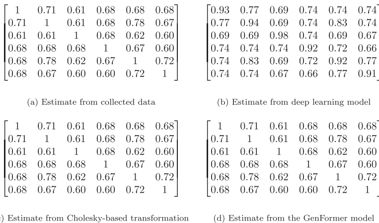
Figure 13. Target spatial correlation matrix of collected wind speeds (a) and various approximations (b), (c), (d). The estimate of the spatial correlation matrix due to the GenFormer model is 12 times more accurate than the estimate produced by the deep learning model without post-processing. On the other hand, the transformation based on Cholesky decomposition preserves the spatial correlation matrix irrespective of the number of locations m .
