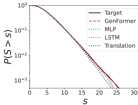
Figure 10. Exceedance probability of S(t) . The relative error in the return period attained by the proposed GenFormer model is approximately an order of magnitude lower than those of the translation model, the MLP, and the LSTM. The GenFormer model can capture higher-order statistical properties of \mathbf{X}(t) beyond the second moment in this example.
