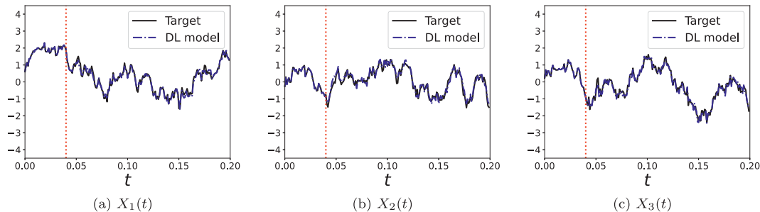
Figure 6. Target versus synthetic time series produced by the deep learning model for inference of m -variate processes. The Transformer-based model produces accurate inference of the target based on the same Markov state sequence.
