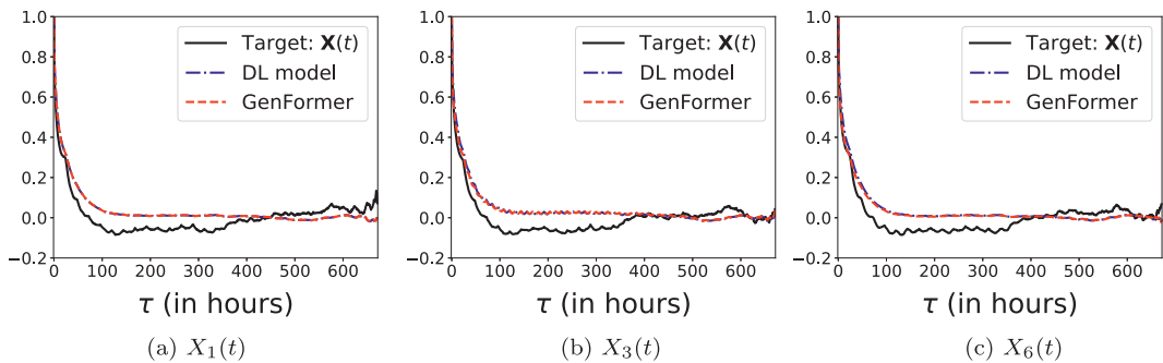
Figure 14. Auto-correlation functions of X_1(t) , X_3(t) , X_6(t) and various approximations. The trained deep learning model provides satisfactory approximations to the auto-correlation functions with the post-processing procedure introducing only minimal and visually-indiscernible deviations.
