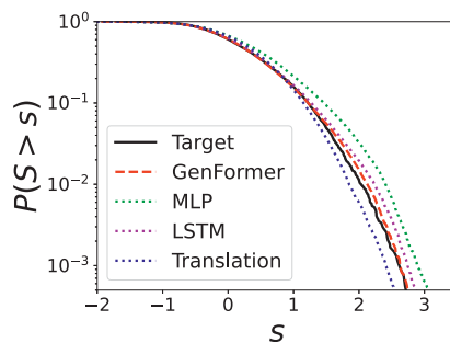
Figure 17. Exceedance probability of S . The estimate obtained from the GenFormer model is 7.6, 4.0, and 2.3 times more accurate than the translation, MLP, and LSTM models. The predictive capabilities of the Transformer-based deep learning model coupled with the statistical post-processing techniques enable the GenFormer model to capture high-order statistical properties.
