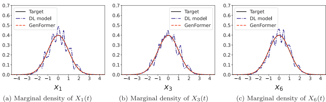
Figure 15. Marginal density estimates of X_1(t) , X_3(t) , X_6(t) . The model post-processing procedure in the GenFormer model, specifically the reshuffling technique, reduces the L_1 relative error by a factor of 11.
