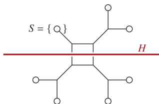
Figure 2. A dual median graph with a half-space H with no principal orientations (circled vertices) on its boundary, and such that the set S of principal orientations in H closest to its boundary do not uniquely identify it (the left side of the vertical hyperplane down the middle would have the same S ).
