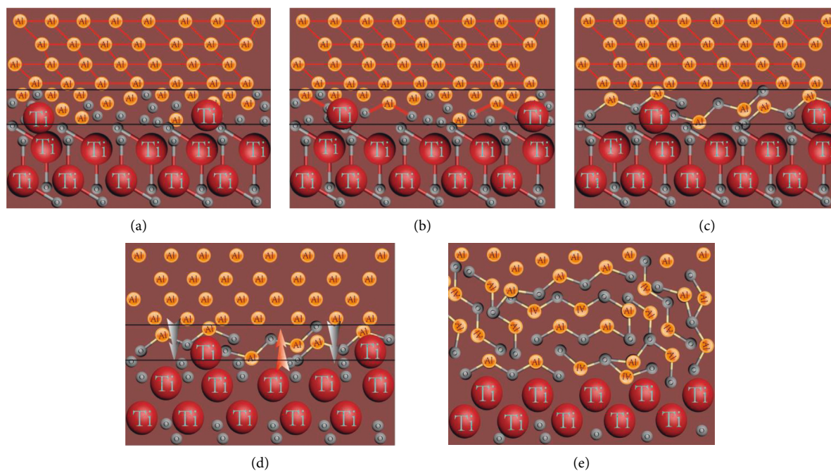
FIGURE 9: Schematics of the main reaction mechanism of the \text{TiO}_2/\text{Al} film. (a) As-deposited. (b) Solid-solid reaction. (c) \text{Al}_2\text{O}_3 barrier. (d) Molten Al. (e) Solid-liquid reaction.
