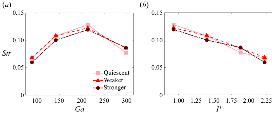
Figure 13. Strouhal number Str = fD/V_t plotted as function of (a) Ga and (b) I^* .
