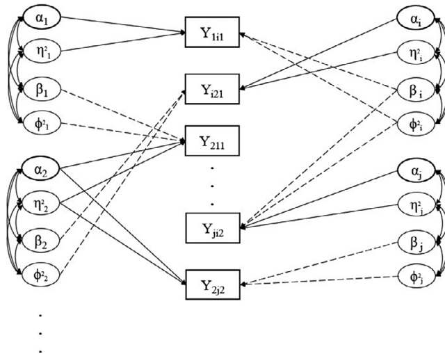
Figure 2. Path diagram representing the network structure of peer grading data.
