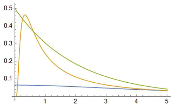
Figure C2. Priors placed under different scenarios on \sigma_1, \dots, \sigma_4, \mu_3, \mu_4 . Note: The blue, orange, and green solid lines indicate, respectively, the half-Cauchy, the inverse-gamma and the exponential priors.
