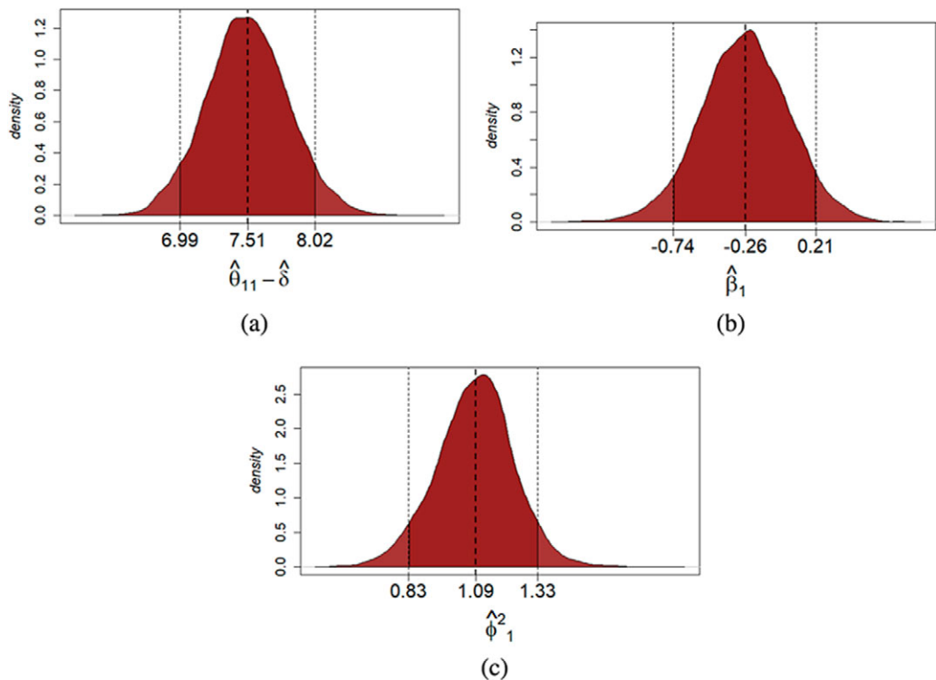
Figure 5. Single assessment example: Posterior distribution of the true score (a), mean bias (b), reliability (c) of student i = 1 . Note: The black dotted lines indicate the 95% quantile-based credible interval and the posterior mean of each estimated parameter.
