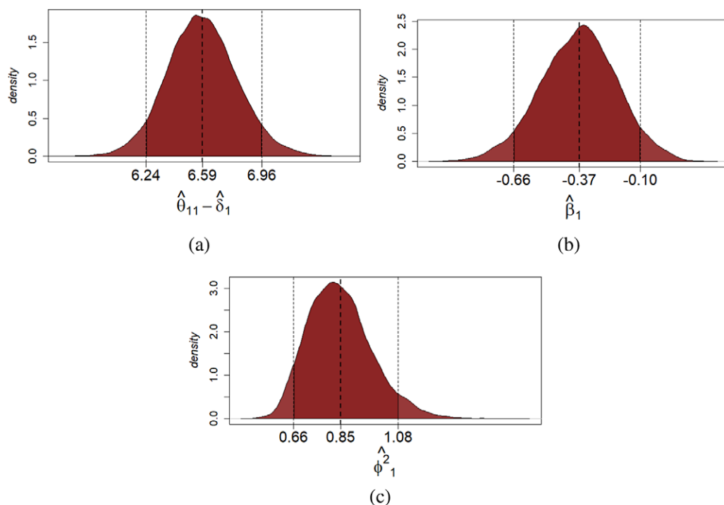
Figure 4. Multiple-assessments example: Posterior distribution of the true score of the first assessment (a), mean bias (b), and reliability (c) of student i = 1 .
