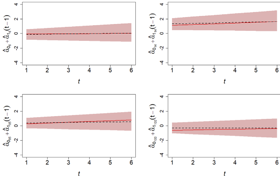
Figure B1. Estimated linear latent growth of a random sample of four students.
