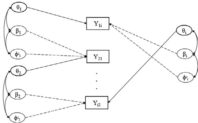
Figure 3. Path diagram representing the network structure of peer grading data for a single assessment.
