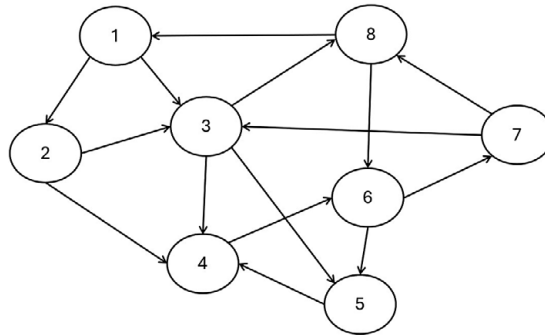
Figure 1. Network diagram representing the network structure of peer grading data.
