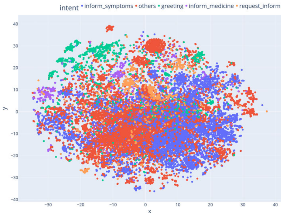
Figure 7. t-SNE visualization for the ninety-nine clusters generated with the Glove embedding model.
