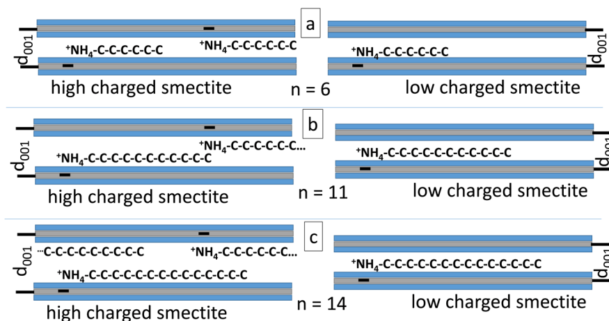
Fig. 4 Schematic representation of the basic concept for determination of the layer charge using the AAM method. The AAM-chains are shown as linear; they are, in fact, zigzag-shaped
