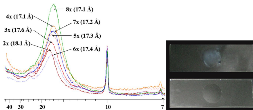
Fig. 3 Effects of various washing steps on the d_{001} spacing of a Bavarian bentonite ( n=13 ; left); right: photographs of glass slides with dried drops of various washing solutions (water/ethanol) in their respective centers. Upper: excess AA present with a cloudy, veil-like appearance; lower: sample after repeated washing, no excess AA is detectable
