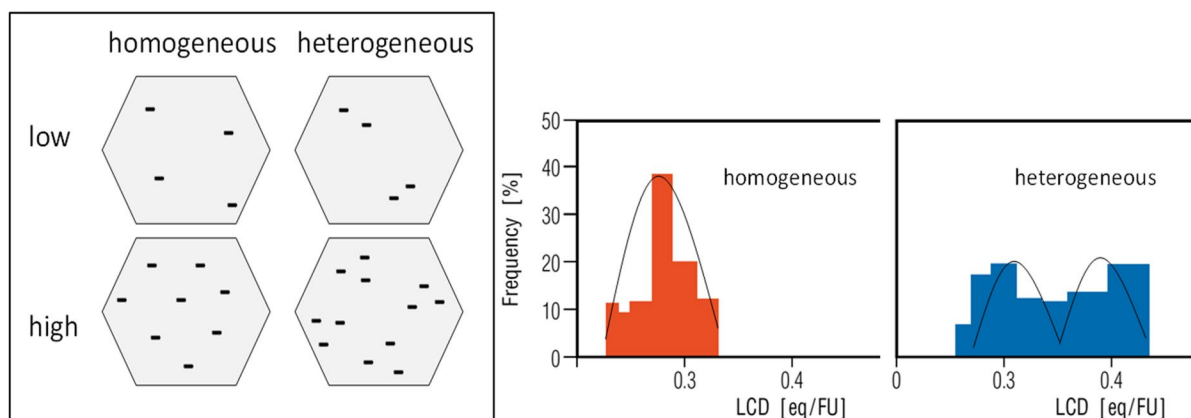
Fig. 6 Left: schematic representation of the option to classify smectites based on AAM results; right: measured data of a more homogeneously charged smectite (red) and a more heterogeneously (close to bimodally) charged smectite (blue)
