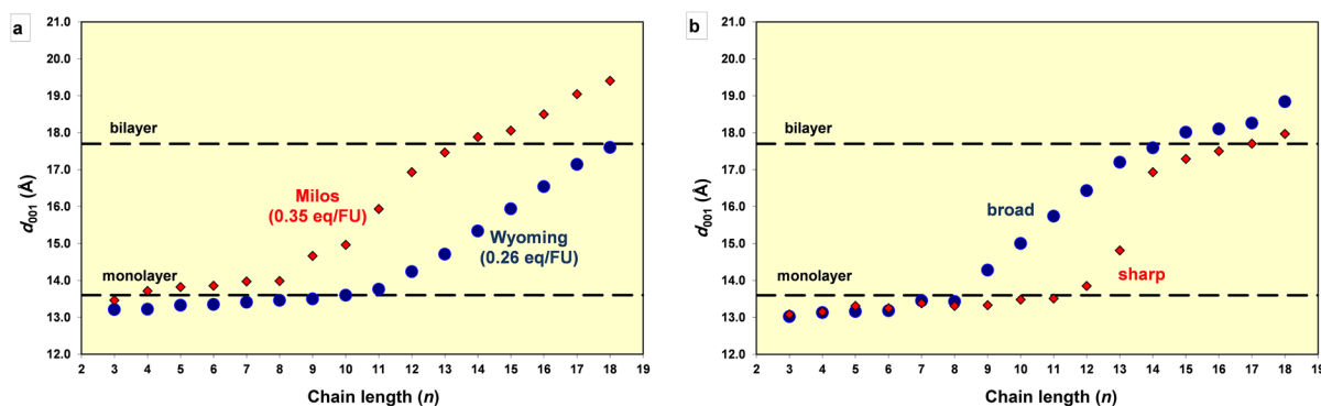
Fig. 5 Examples of peak migration curves in the AAM method: a low- and high-charge; b broad and sharp charge distributions
