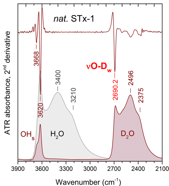
Fig. 13 Separation of structural OH ( \text{OH}_s ) and \text{H}_2\text{O} (as \text{D}_2\text{O} ) absorbance spectra of STx-1 montmorillonite (in as-received interlayer cation form) by in situ deuteration at ambient temperature. The position of the sharp \nu\text{O}-\text{D}_w mode (highlighted red) is determined by the 2nd derivative minima (4 \text{cm}^{-1} resolution, \Delta\nu=2\text{ cm}^{-1} , Savitzky-Golay 13 pt smoothing, as in Kuligiewicz et al., 2015b). The ATR spectrum of the sample prior to deuteration is included for comparison (shaded gray)
