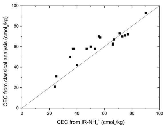
Fig. 7 Example of the relationship between the CEC calculated from \text{NH}_4^+ methods and the CEC measured by the classical method. The samples are from soil series and from various kaolinite-smectite mechanical mixtures. Data adapted and modified from Petit et al. (1998)
