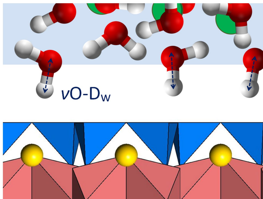
Fig. 12. Schematic representation of the dangling O-H w /O-D w bonds in the interlayer of smectite (drawing not to scale). For details, see text
