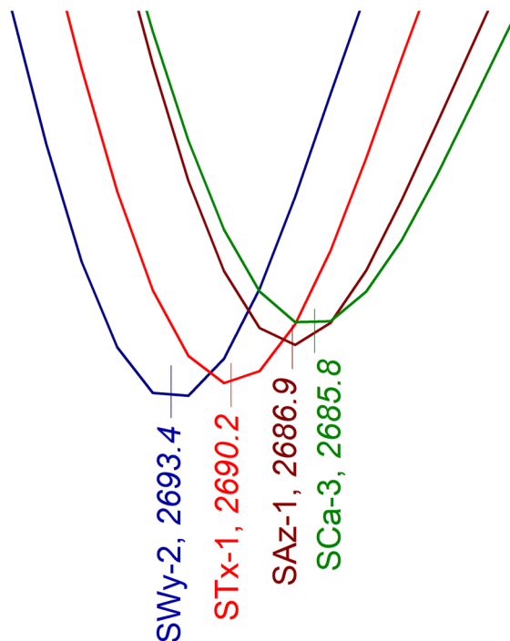
Fig. 14 Position of the \nu\text{O}-\text{D}_w 2 nd derivative minima of SWy-2, STx-1, SAz-1, and SCa-3 montmorillonites in their as-received cation forms (cf. Figure 13)
