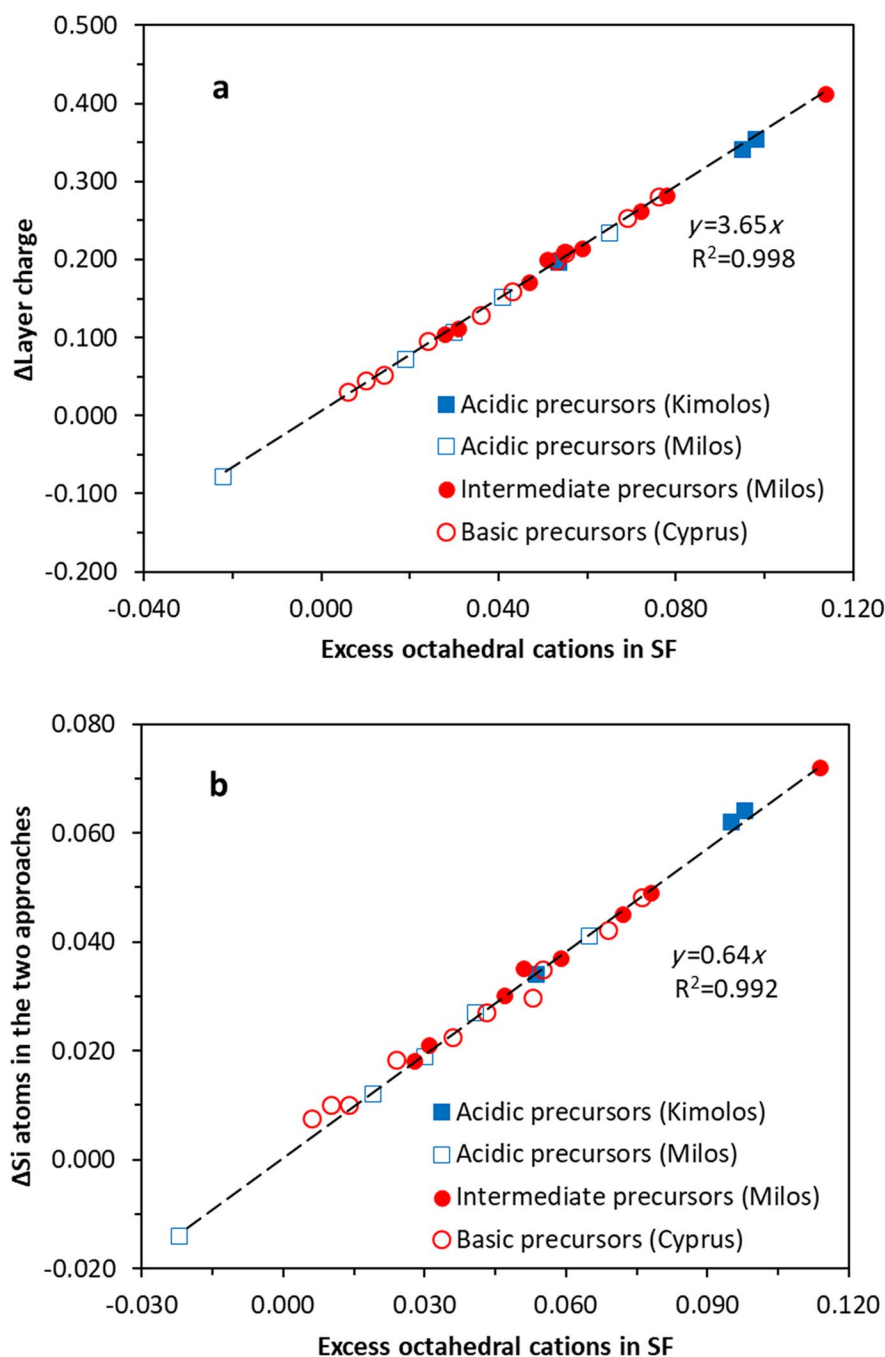
Fig. 1 Excess octahedral cations (e/huc) calculated with the fixed anionic charge approach vs a difference in layer charge calculated by the two approaches and b the difference in Si atoms calculated by the two approaches
