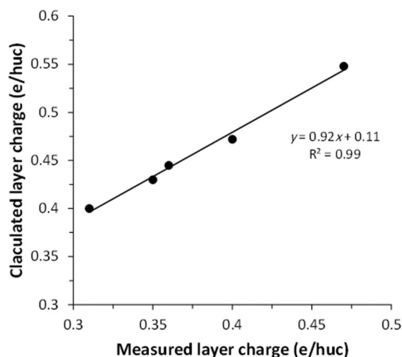
Fig. 11 Correction of the layer charge for smectites with a predominantly tetrahedral charge
