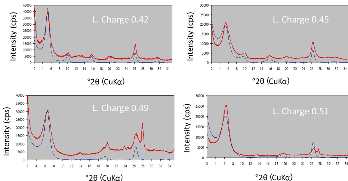
Fig. 10 Simulation of XRD traces of K-saturated and EG-solvated smectites using the LayerCharge program. Red=experimental XRD trace, blue=computed XRD trace (data from Makri, 2011)
