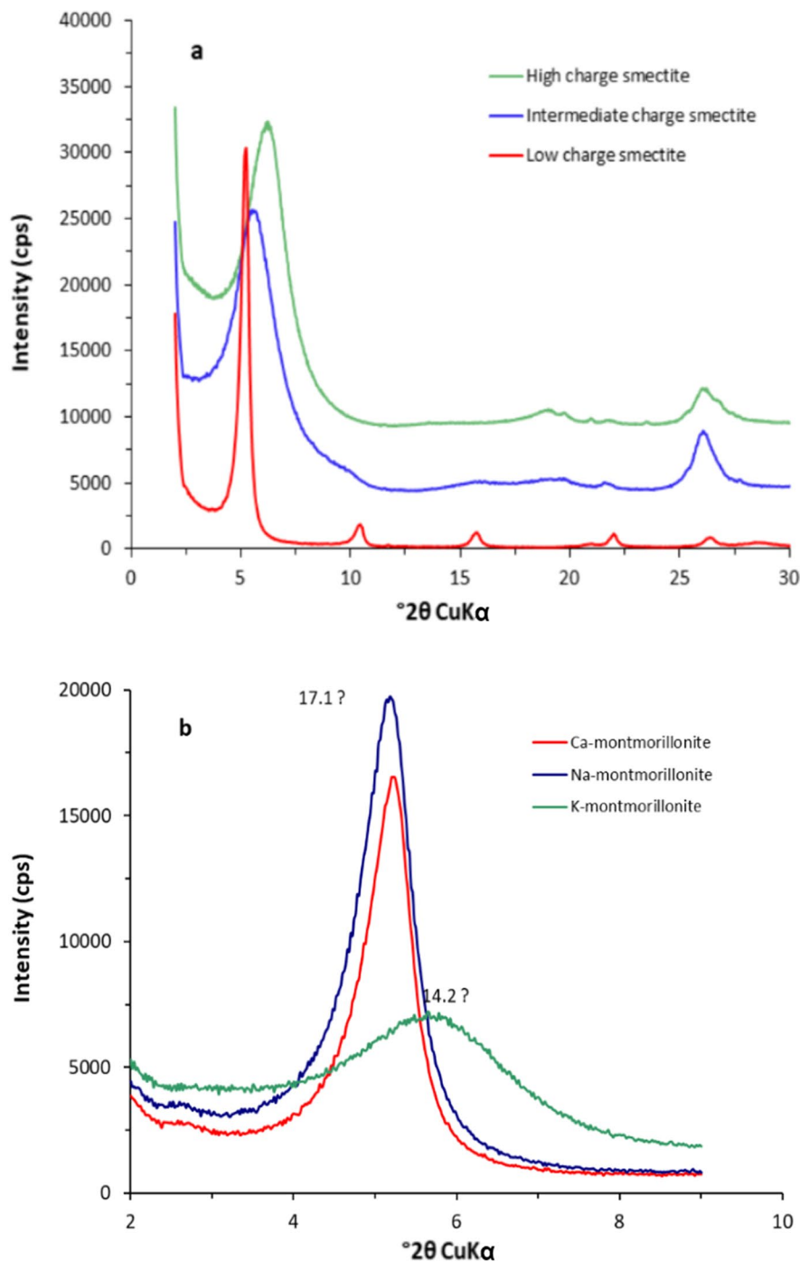
Fig. 9 a XRD patterns of K-saturated, EG-solvated smectites with low, intermediate, and high layer charge. b XRD traces of EG-solvated SAz-1 montmorillonite saturated with K, and back-saturated with Na and Ca ions
