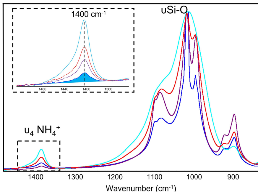
Fig. 8 Example of a normalized IR spectrum (see text) of smectite SAz-1 mixed with various weight percentages of kaolinite KGa-1 (0%, light blue line; 25%, red line; 50%, purple line; 75%, blue line) in the regions of the \nu_4 \text{NH}_4^+ bands and \nu\text{Si-O}
