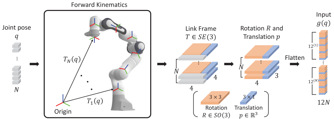
Figure 2. An illustration of the link SE(3) configuration space representation mapping g . The joint configuration q is mapped to the collection of link frames T_i(q) and transformed to an input vector g(q) .
