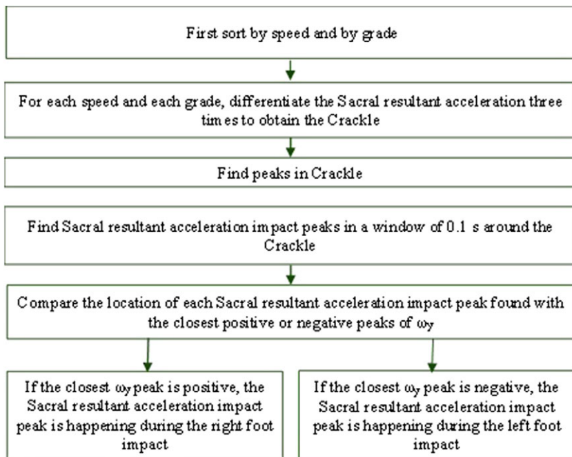
Figure 5. Flow chart of detecting right and left initial contact from the sacral IMU using both crackle and angular velocity about the anterior-posterior axis.
