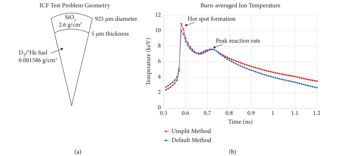
FIGURE 7: An ICF test problem based on an OMEGA capsule experiment: (a) the initial geometry of the capsule and (b) the calculated burn-averaged ion temperature from separate highly resolved 1D simulations using the default and unsplit hydrodynamic methods in xRAGE.
