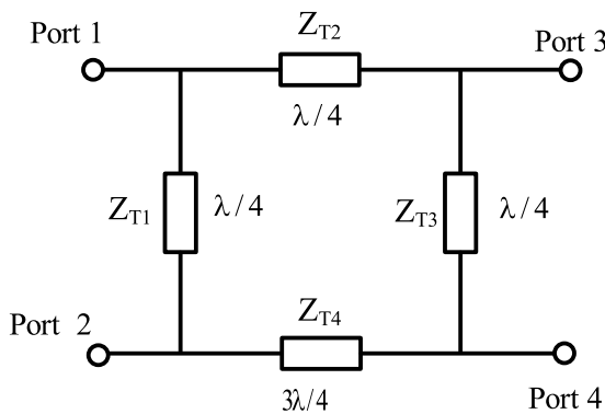
Figure 4. The conventional single-band rat-race coupler [29].
