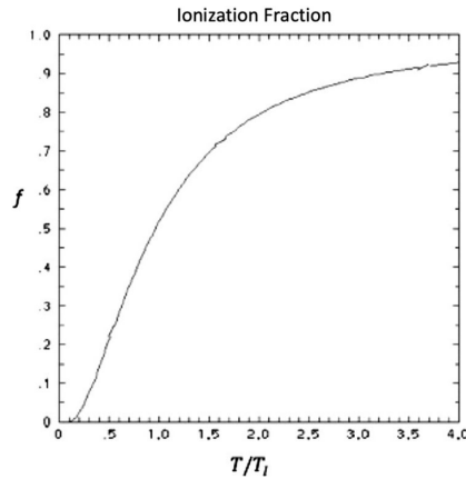
FIGURE 10. Fractional ionization versus T/T_I(n) based on (1.321).
