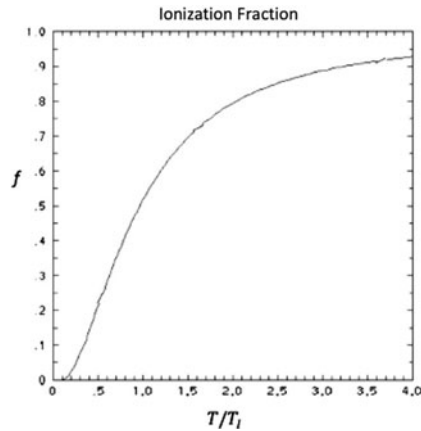
FIGURE 10. Fractional ionization versus T/T_1(n) based on (1.321).
