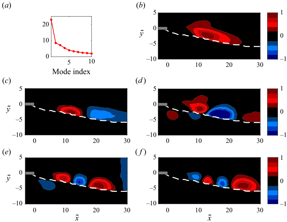
Figure 24. POD analysis of the G5 case of table 3 . (a) POD modes energy distribution (%). (b–f) Leading modes (1st to 5th, respectively, each scaled with respect to its maximum). In each plot, the splitter plate is highlighted in grey, and the mean interface location is denoted by the white dashed line.
