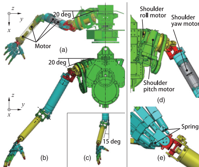
Figure 5. Three-dimensional computer-aided design image of the ibuki 's upper body: (a) top view; (b) front view; (c) forearm; (d) shoulder; and (e) wrist joint.
