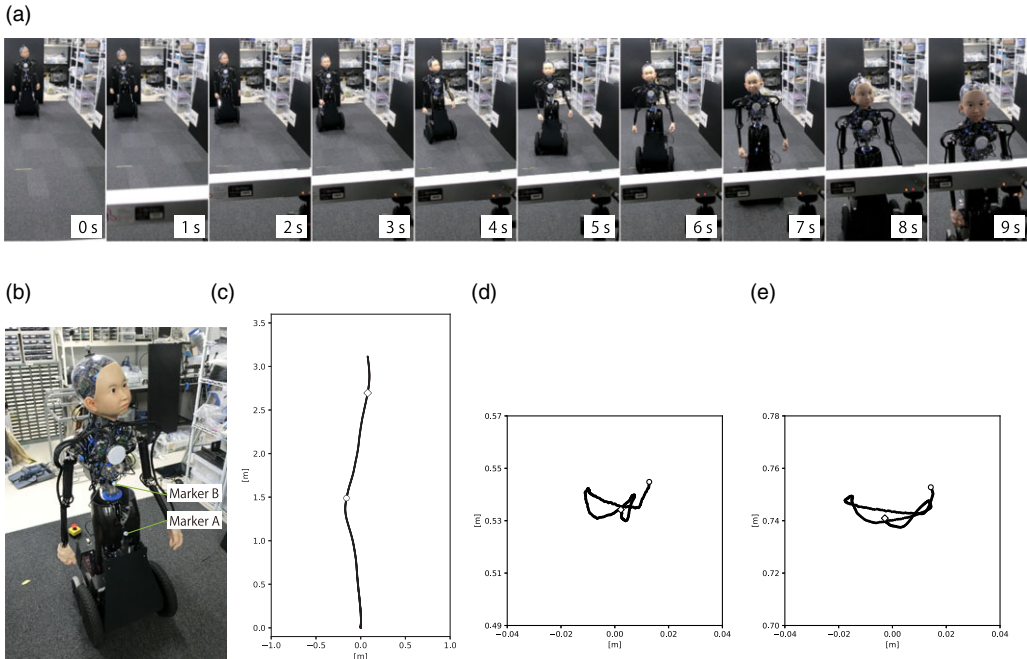
Figure 17. The measurement of the gait-induced upper body motion: (a) time series photographs of the motion; (b) arrangement of the reflection markers; (c) trajectory of the ibuki 's movement on the horizontal plane; (d) trajectory of the marker A; and (e) trajectory of the marker B.
