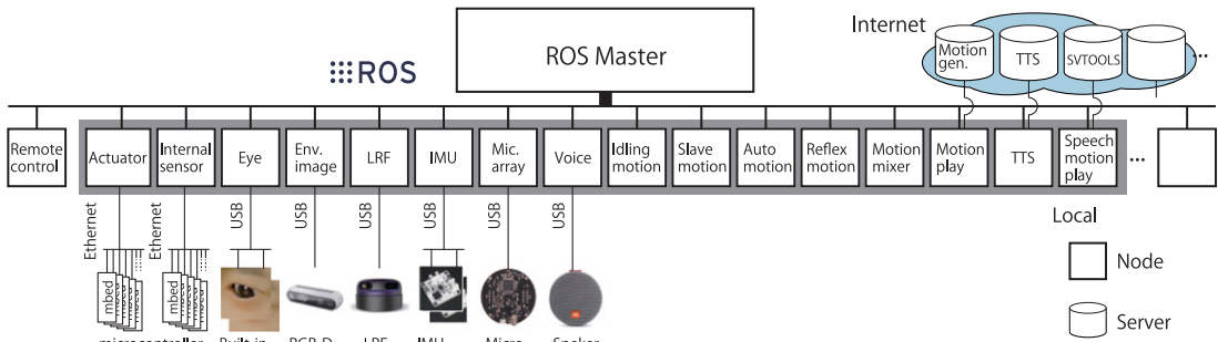
Figure 10. The ROS-based software package for androids called “SILVA”.
