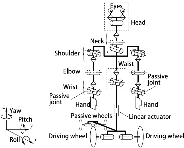
Figure 2. The mechanical structure of ibuki . The wrist roll axes of both arms are specified as passive joints. Mechanical springs are attached to each joint.
