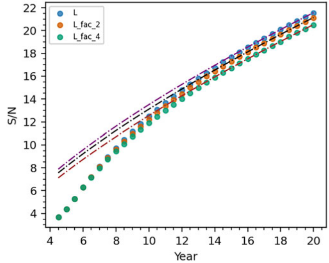
Figure 11. Evolution of S/N with time span of MPTA. We show the S/N variations for simulated datasets up to 20 yr for three observing strategies: standard L-band (L), twice cadence observations (L_fac_2), and quadrupled cadence observations for best MSPs (L_fac_4). The S/N is estimated for an SGWB self-noise amplitude at 5 \times 10^{-15} , that is, the CURN amplitude of MPTA. The dashed lines represent a power law model fit to the last four years of the dataset and indicate a transition from the weak signal regime towards a strong signal regime for the SGWB.
