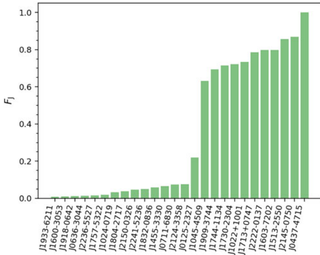
Figure 1. Fraction of jitter-limited observations ( F_j ) per pulsar in MPTA. Out of the 41 MSPs, 15 pulsars are not included in this analysis as none of the observations were jitter-limited according to our definition. The pulsars are sorted by the fraction, and PSR J0437–4715 has 100% observations that are jitter-limited.
