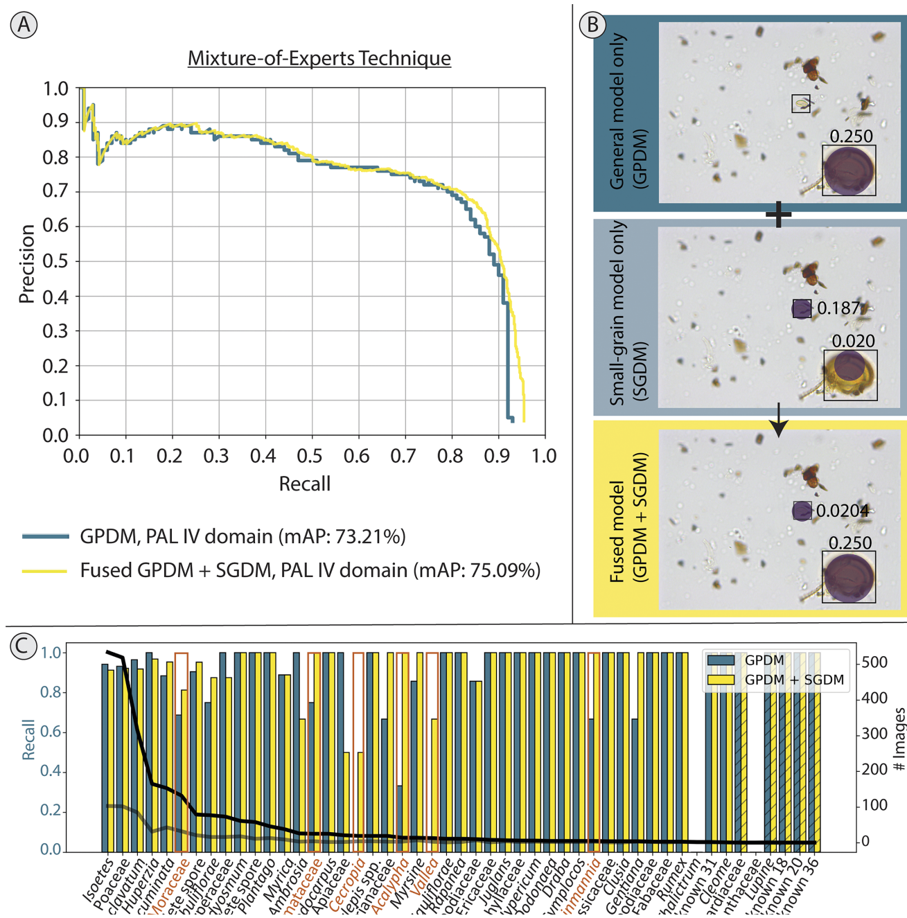
Figure 5. Results of general pollen detection model (GPDM), application of the mixture-of-experts technique, and application of transfer learning. A , For the mixture-of-experts technique, comparison of the blue (GPDM) and yellow (fused model) curves shows how the addition of an expert model trained only on small pollen grains improves maximum model recall from 93% to 95%. B , Comparison of detections from the general model, the small-grain model, and the fused model. Boxes in each panel indicate ground-truth labels, and circles indicate detections. The color of the detections is arbitrary. Confidence scores are shown adjacent to each detection. small-grain detection model (SGDM) confidence scores in the fused model have been calibrated as described in the text. A validation-set image stack containing a Cecropia pollen grain and Isoetes spore was fed into the two models. The GPDM detected the Isoetes spore with high confidence but missed the Cecropia grain. The SGDM was able to detect the Cecropia grain but had poor localization accuracy and low confidence for the Isoetes spore. The fused model kept both detections. C , Blue and yellow bars indicate model recall by taxon for the GPDM and the fused (GPDM + SGDM) models respectively (left y-axis). The black and gray lines indicate the abundance distribution of taxa in the GPDM training and validation datasets, respectively (right y-axis). Both models were thresholded at the confidence value that yielded 20% precision. The taxa highlighted in orange are particularly small-grained taxa, which have low rates of detection relative to the number of training examples. Hatched bars indicate taxa that had no training examples but were in the validation set and detected by the detector. mAP, mean average precision; PAL IV.
