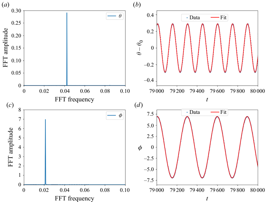
Figure 19. Fitting the time dependence given by (3.4) to the numerical data for the orientation angles \theta and \phi in the rocking mode with B = 14\,098 . (a,c) The FFT analysis of \theta and \phi . (b) The fit of \theta - \theta_0 is performed with one dominant FFT frequency 2\omega_r . (d) The fit of \phi is performed with one dominant FFT frequency \omega_r .
