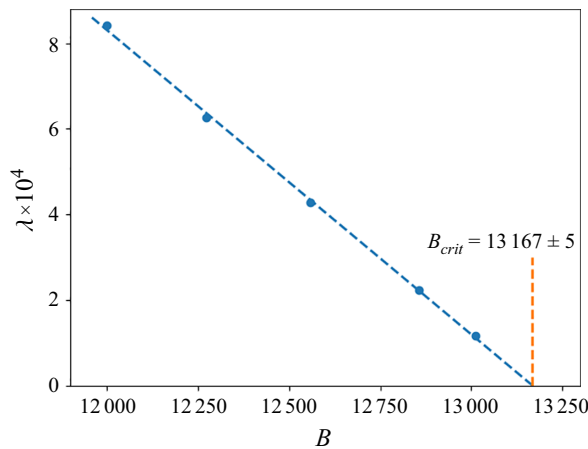
Figure 16. The growth rate \lambda in (4.1) is a linear function of B , enabling estimation of B_{crit} = 13\,167 for the transition between the frozen rotating and tilted modes.
