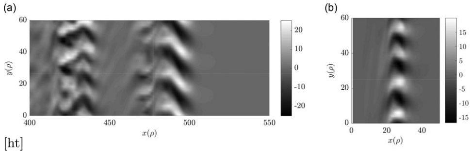
FIGURE 4. (a) Density plot of electrostatic potential (in units of T_0\rho_s/eR ) at the outboard mid-plane versus radial ( x ) and binormal ( y ) coordinate for standard-box gyrokinetic simulations for S = 0.35 . This is the state at t = 250a/c_s in this simulation (cf. Figure 1a). (b) Density plot of electrostatic potential at the outboard mid-plane versus radial ( x ) and binormal ( y ) coordinate for standard-box gyrokinetic simulations for S = 0.75 . In both cases the bursts are propagating in the positive x direction.
