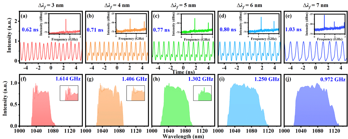
Figure 5. Experimental results under different \Delta\lambda_f . (a)–(e) Pulse train; inset, RF spectrum. (f)–(j) Spectra; inset, zoom-in of the CW state.
