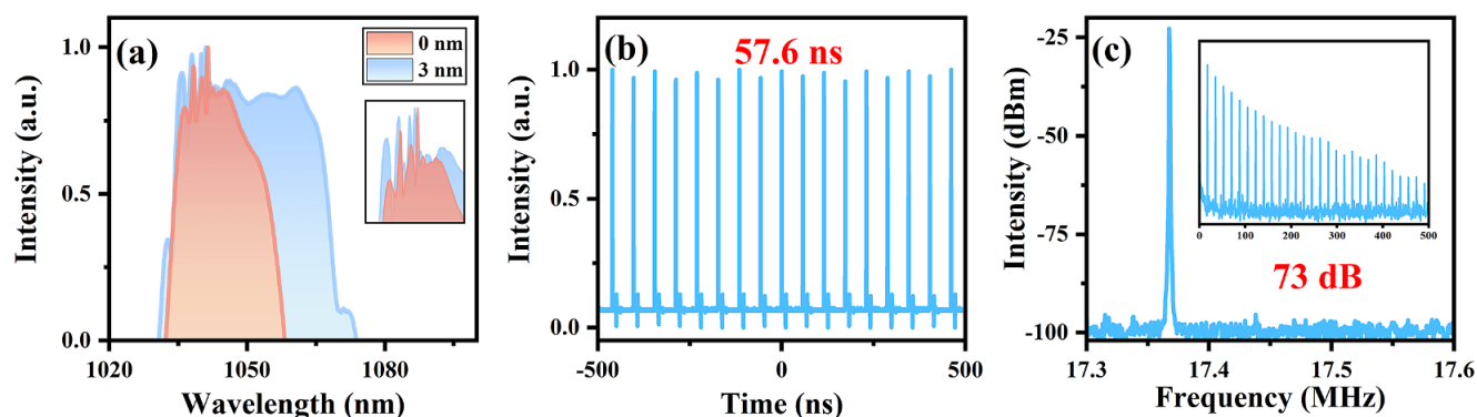
Figure 2. Experiment results. (a) Spectra: red is the mode-locked spectrum when the \Delta\lambda_f is 0 nm; blue is the mode-locked spectrum when the \Delta\lambda_f is 3 nm; inset shows the zoom-in of the CW state. (b) Pulse train. (c) RF spectrum.
