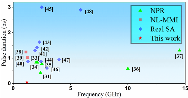
Figure 8. Overview of GHz harmonic mode-locking in different configurations [33–48].
