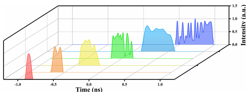
Figure 3. Evolution of the pulses with increasing pump power.
