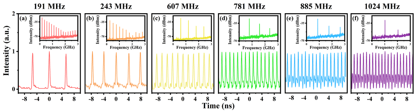
Figure 4. HML pulse train and RF spectrum: (a) 11th, (b) 14th, (c) 35th, (d) 45th, (e) 51st and (f) 59th harmonic orders.
