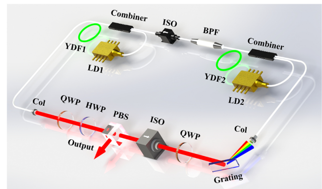
Figure 1. Schematic setup of the MO for generating GHz harmonic mode-locking. Col, collimator; YDF, Yb-doped fiber; BPF, bandpass filter; QWP, quarter-wave plate; HWP, half-wave plate; PBS, polarization beam splitter; ISO, isolator; LD, laser diode.
