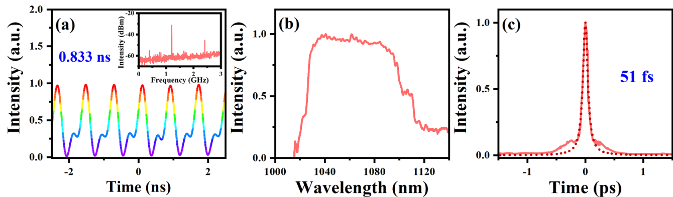
Figure 6. Experimental results. (a) Pulse train; inset, RF spectrum. (b) Spectrum. (c) Autocorrelation trace.
