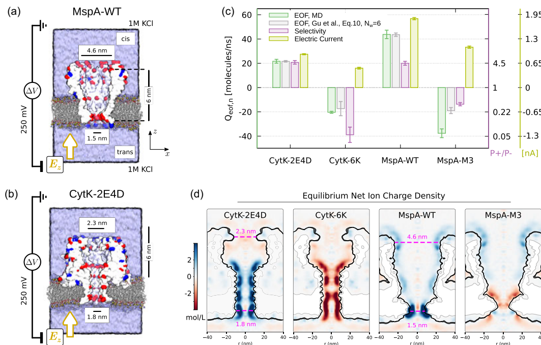
Figure 4. Biological nanopores MspA and CytK. (a,b) Simulation set-up of atomistic simulation. The pores are represented as isosurfaces extracted from a volumetric Gaussian density map (QuickSurf representation in Krone et al. (2012)) and it is cut along a vertical plane to show the pore lumen. Exposed residues carrying a net charge are represented in red (negative) and blue (positive). The pore are embedded in a lipid membrane. Water and ions are omitted for clarity. We represented the cation selective pores (MspA-WT and CytK-2E4D) that exposed negative residues towards the pore lumen. (c) Selectivity, total electric current and EOF from MD simulations for cation and anion selective MspA and CytK mutants. The prediction from (11) obtained using the cation and anion currents from MD and N_w = 6 are reported in grey. (d) Equilibrium ( \Delta V = 0 ) MD ionic net charge density distributions for the four nanopores. The maps are obtained transforming the original Cartesian maps in a cylindrical coordinate system and then averaging on the angular coordinate. To highlight the pore shape, we represented contour levels of the water density corresponding to 0.95, 0.5 and 0.25 \rho_{bulk} , with \rho_{bulk} being the bulk water density. Confidence intervals in (c) were obtained using a block average with each block corresponding to 10 ns. For derived quantities (as selectivity) we applied uncertainty propagation rules. For the Gu et al. (2003) prediction, we used (6) instead of (10) to reduce the error propagation. As for figure 3 to compact multiple data on the same plot, three different scales are used for the vertical axis (linear for Q_{eof,n} , logarithmic for P_+/P_- and total current). The original data are reported in table S3 of the supporting information.
