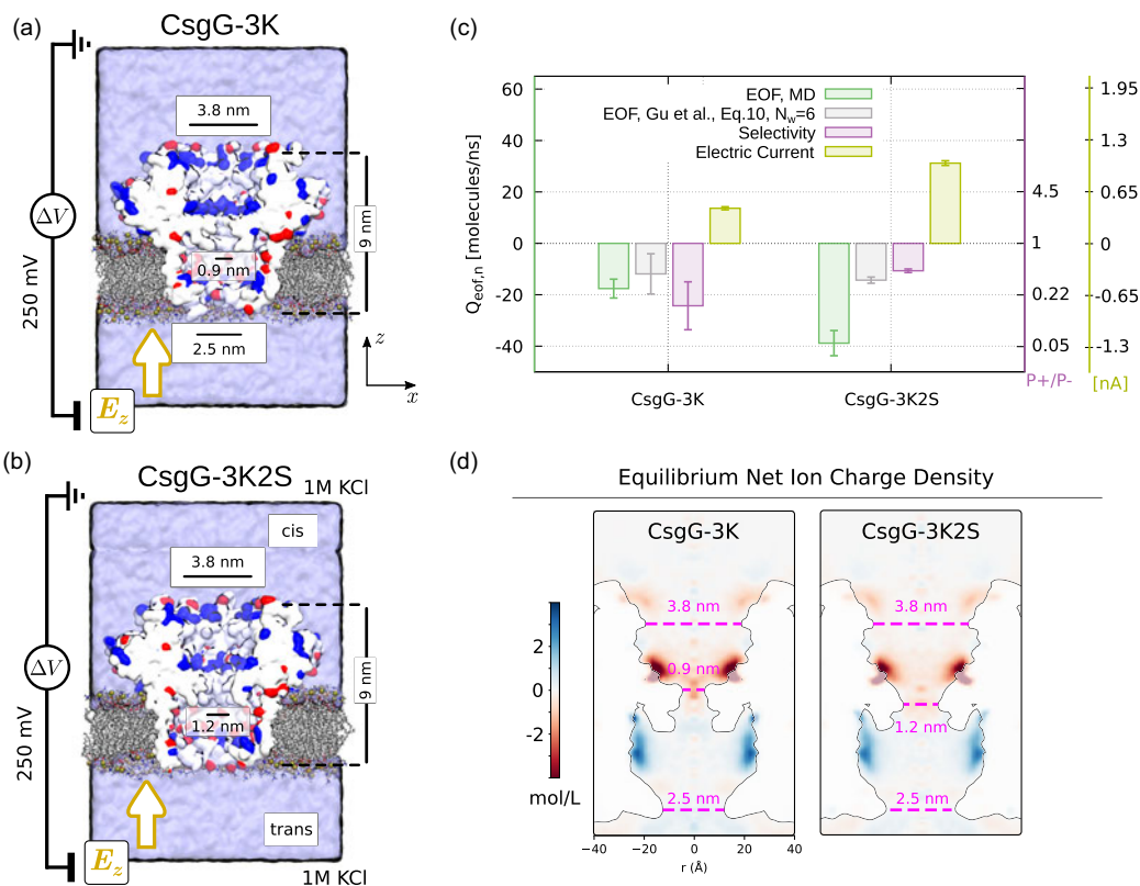
Figure 5. Biological nanopore CsgG. (a,b) Picture showing the set-up of atomistic simulation. The main structural difference between the two mutants is the larger constriction of the CsgG-3K2S compared with the CsgG-3K. In particular, the CsgG-3K mutant presents three mutations (D43K, G46K, Q62K), while the CsgG-3K2S presents the same three plus two additional ones (Y51S, F56S) located in the constriction. The total charge of the two pores is the same. The pores are represented as in figure 4. (c) Selectivity, total electric current and EOF from MD simulations as in figure 4. The prediction from (11) obtained using the cation and anion currents from MD and N_w = 6 are reported in grey. (d) Equilibrium ( \Delta V = 0 ) MD ionic net charge density distributions are calculated as in figure 4. To highlight the pore shape, we represented the contour level of the water density corresponding to 0.5 \rho_{bulk} , with \rho_{bulk} the bulk water density. Confidence intervals in (c) were obtained using a block average with each block corresponding to 10 ns. For derived quantities we applied uncertainty propagation. As for figure 3 to compact multiple data on the same plot, three different scales are used for the vertical axis (linear for Q_{eof,n} , logarithmic for P_+/P_- and total current). Original data are reported in table S3 of the supporting information.
