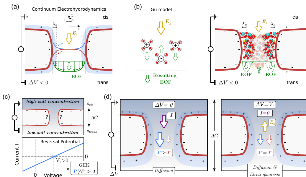
Figure 1. Electro-osmotic flow in nanopores and its connection with selectivity. (a) Sketch of the continuum electrohydrodynamic model for EOF in cylindrical nanopores. A typical nanopore sensing device is constituted by a single nanopore embedded in a membrane. The nanopore connects two reservoirs that, as usual in the electrophysiology and nanopore sensing field, are here indicated as cis and trans. One of the two reservoirs is grounded (in our case, cis) and a voltage \Delta V is applied at the trans side. Moreover, different ion concentrations can be present in the two reservoirs resulting in a concentration difference \Delta C_i , with i the ion species. Here, we consider only the case when the electrolyte is of the same kind at the cis and trans sides and it is obtained dissolving a salt; consequently, the salt concentration difference \Delta C is the only relevant parameter to define the concentration differences of all the ions. Fixed charges are present at the nanopore surface, resulting in an equilibrium ( \Delta V = 0 , \Delta C = 0 ) distribution of ion charge in the pore. Under a voltage load \Delta V , this charge accumulation typically results in two effects: (i) the pore is selective for positive (cation) or negative (anion) species and (ii) an EOF sets in. The EOF is due to the net force that the ions transfer to the fluid under an external \Delta V . If the pore is negatively charged (as in the figure), positive ions accumulate in the pore, and the axial component of electric field acts on the positive ions that, in turn, transfers momentum to the fluid putting it in motion. Panel (a) refers to a condition where \Delta C = 0 so that the Debye length \lambda_D is the same in any region of the system. (b) Pictorial view of the Gu et al. (2003) model, showing the EOF originated from the transport of the water molecules around each ion. The main limitation of the model is that it does not account for the viscous drag that will put in motion the fluid also in the uncharged portion of the pore lumen. (c) The GHK model: selectivity measurement from reversal potential. The EOF in single nanopores cannot be directly measured. Moreover, also cation and anion contributions to the total current I are not directly accessible. An accessible quantity is, instead, the reversal potential V_r that is the applied voltage at which, in presence of a \Delta C , the electric current is zero. (d) Sketches of the directions of the ionic flows in the case of a 1 : 1 electrolyte for (i) \Delta V = 0 and (ii) \Delta V = V_r .
