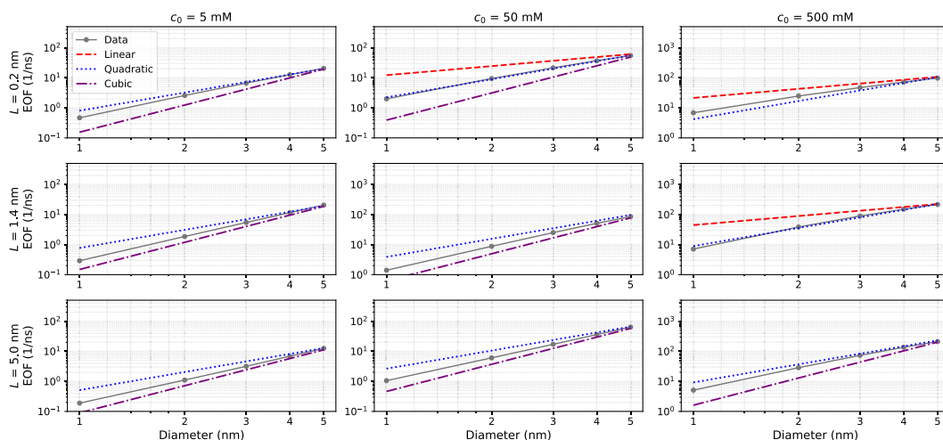
Figure 3. The EOF scaling from PNP-S simulations. The EOF as a function of pore diameter for three different electrolyte concentrations ((a,d,g), (b,e,h) and (c,f,i)) and three pore lengths ((a–c), (d–f) and (g–i)). Each plot corresponds to a specific combination of c_0 = 5, 50, 500 mM (from (a,d,g) to (c,f,i)) and L = 0.2, 1.4, 5 nm (from (a–c) to (g–i)). The markers represent the raw data, while the red dashed curves, the blue dotted curves and the dot–dashed purple curves are the linear, quadratic and cubic trends, respectively. Only relevant trends, to guide the eyes, are shown.
