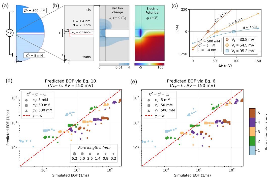
Figure 2. The Poisson–Nernst–Planck–Stokes systems (PNP-S) simulation of electrohydrodynamics in cylindrical nanopores. (a) Sketch of the system set-up. The pore is negatively charged. The salt concentrations and electric potentials of the reservoirs are controlled by imposing appropriate boundary conditions at the reservoir hemispherical boundaries, details in Supplementary figure S2. (b) Zoom showing representative solutions for the net ion charge density \rho_e = e(c_+ - c_-) and electric potential \phi in the nanopore region, for C^t = 5 mM, C^c = 500 mM KCl and \Delta V = 150 mV. (c) The IV curves for reversal potential simulations for three nanopores of length L = 1.4 nm and varying diameters, d = 1, 3, 5 nm. The potential V_r is obtained interpolating the \Delta V for which the electric current I is zero. Data points computed at \Delta V = 0, 50, 150 mV are marked. (d-e) Comparison of simulated EOF with predictions from (10) and (6) for various geometries and concentrations. The EOF simulations are performed for \Delta V = 150 mV, and setting an identical electrolyte concentration in the two reservoirs C^t = C^c = c_0 . Datapoints are coloured by the pore radius, and the marker symbols represent the reservoir concentrations, as indicated by the right-hand side colour bar and the inset legend; the marker size is proportional to L . The predictions via (10) are estimated computing the selectivities P_+/P_- from (4), with the reversal potentials V_r interpolated for each geometry as for panel (c), see Supplementary figure S5. Prediction via (6) are computed using the ionic flows Q_{\pm} directly measured together with the EOF. For completeness, the data for the simulated currents and flows are reported on Zenodo, doi:10.5281/zenodo.14916088.
