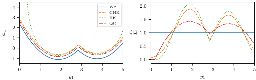
Figure 4. One-dimensional slices of computational results from Figure 3 along [0, L] \times \{0.375 L\} with L = 5 . Left: \phi_w for optimal w \in \mathbb{R}^M . For models (a), (b), and (d), \phi_w is piecewise quadratic; for (c) the profile is determined by c_{HK} and \phi_w = \infty on R \neq \emptyset . Right: Optimal density \frac{d\rho}{d\mu} , where \frac{d\rho}{d\mu} = (F^*)'(-\phi_w) on \Omega \setminus R and 0 elsewhere by (3.4b). For (a) the density is constant, for (b) it is piecewise Gaussian, for (c) it is piecewise given by \cos(d(y, x_i))^2 on \Omega \setminus R and 0 on R , and for (d) it is given by truncated parabolooids.
