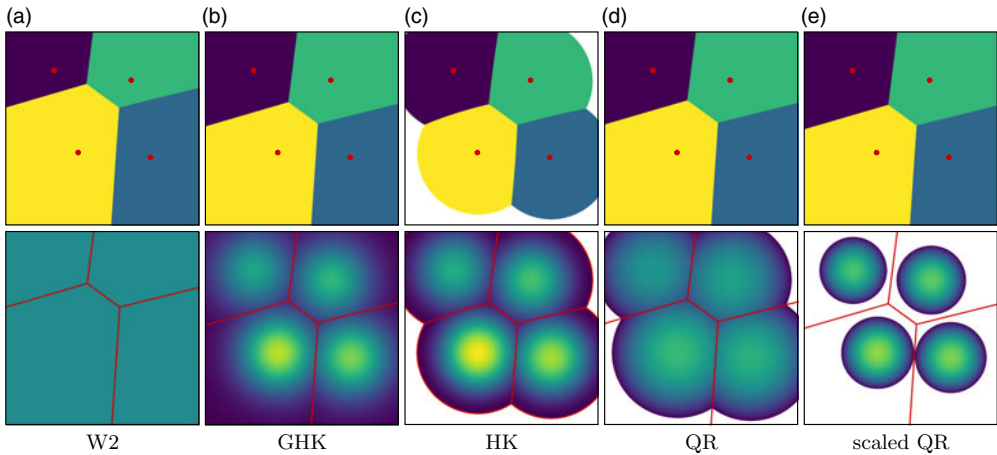
Figure 3. Semi-discrete transport between the Lebesgue measure on \Omega = [0, L]^2 , L = 5 and a discrete measure with M = 4 Dirac masses of locations (x_1, x_2, x_3, x_4) = L \cdot ((0.375, 0.375), (0.75, 0.35), (0.65, 0.75), (0.25, 0.8)) and weights (m_1, m_2, m_3, m_4) = |\Omega| \cdot (0.38, 0.29, 0.19, 0.14) . Top row: optimal cells \{C_i(w)\}_{i=1}^M ; the residual set R is represented by white; location of the discrete points (x_1, \dots, x_M) is indicated with red dots. Bottom row: optimal marginal \rho (identical colour scale in all figures; regions with \frac{d\rho}{d\mu}(x) = 0 are white for emphasis) and boundaries of cells \{C_i(w)\}_{i=1}^M (red) are shown for models (a)–(b) from Examples 2.9 and 3.14. Figure (e) shows the same model as (d), only with c(x, y) = [d(x, y)/2]^2 instead of c(x, y) = d(x, y)^2 ; on some cells \text{spt } \rho is now strictly bounded away from the boundaries of C_i(w) .
