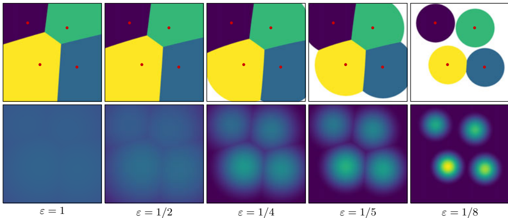
Figure 2. Semi-discrete Hellinger–Kantorovich transport on \Omega = [0, 1]^2 (using the same values for x_i/L and m_i/|\Omega| as in Figure 3) for different length scales \varepsilon . Top row: optimal cells \{C_i(w)\}_{i=1}^M ; the residual set R is represented by white; location of the discrete points (x_1, \dots, x_M) is indicated with red dots. Bottom row: optimal marginal \rho (using the same colour scale for all images). For large \varepsilon , the behaviour is similar to that of the standard semi-discrete Wasserstein-2 distance. As \varepsilon decreases, the effects of unbalanced transport become increasingly prominent.
