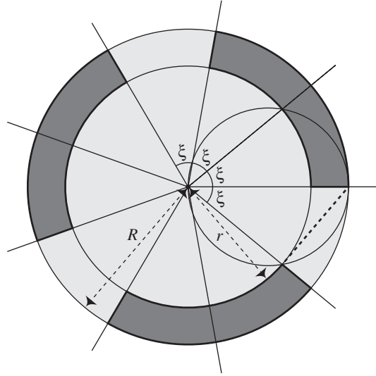
FIGURE 3: The definition of a pearl.
