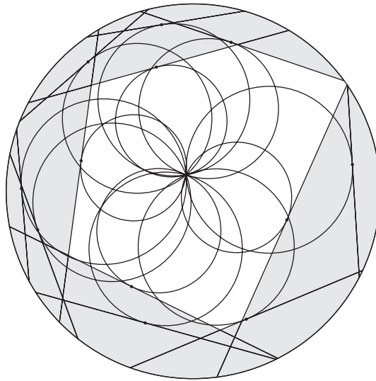
FIGURE 6: Several points and their separators.
