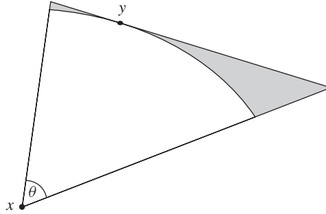
FIGURE 5: The definition of a wedge.
