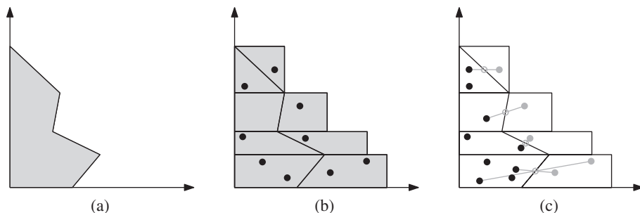
FIGURE 9: (a) A t -shape S . (b) Covering S to obtain a shape S' and uniformly distributing points in S' . (c) Reflecting the points in S' to obtain points uniformly distributed in S .
