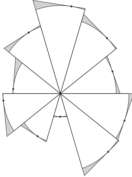
FIGURE 7: Sectors, red points, and blue wedges.
