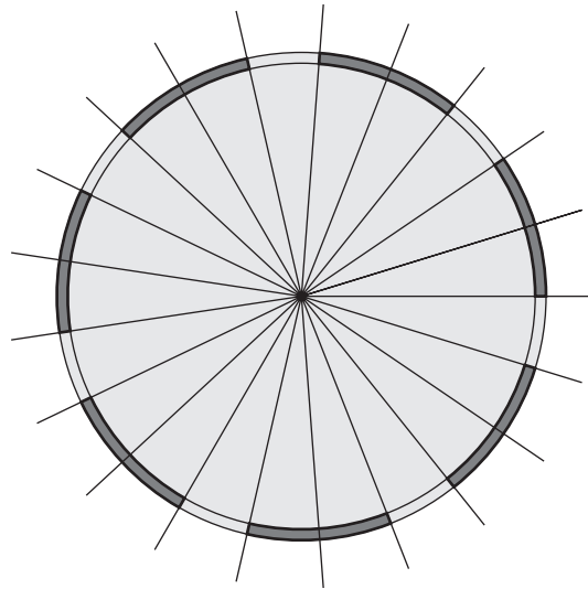
FIGURE 4: The shaded regions define a (7, r) -tiara.
