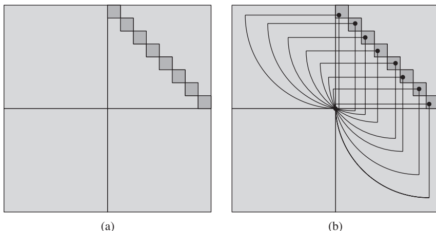
FIGURE 8: An (8, r) -staircase.
