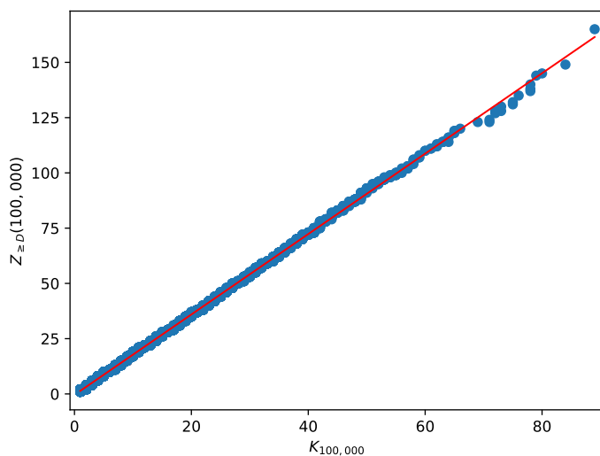
FIGURE 2. Q–Q plot for Z_{\geq D}(100\,000) and K_{100\,000} using a sample size of 10 000.
