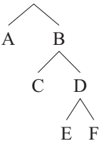
(8) Feature geometry
