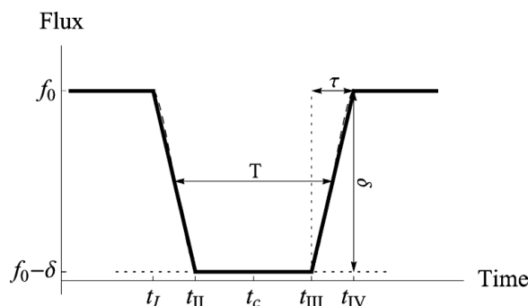
Figure 1. Linear model for a transit light curve with negligible limb darkening. Dashed line shows the physical light curve approximated by the linear model.
