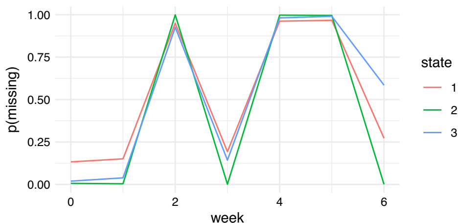
Figure 5. Predicted probability of missing IMPS Item 79 ratings by week for each state in the three-state MNAR hidden Markov model.
