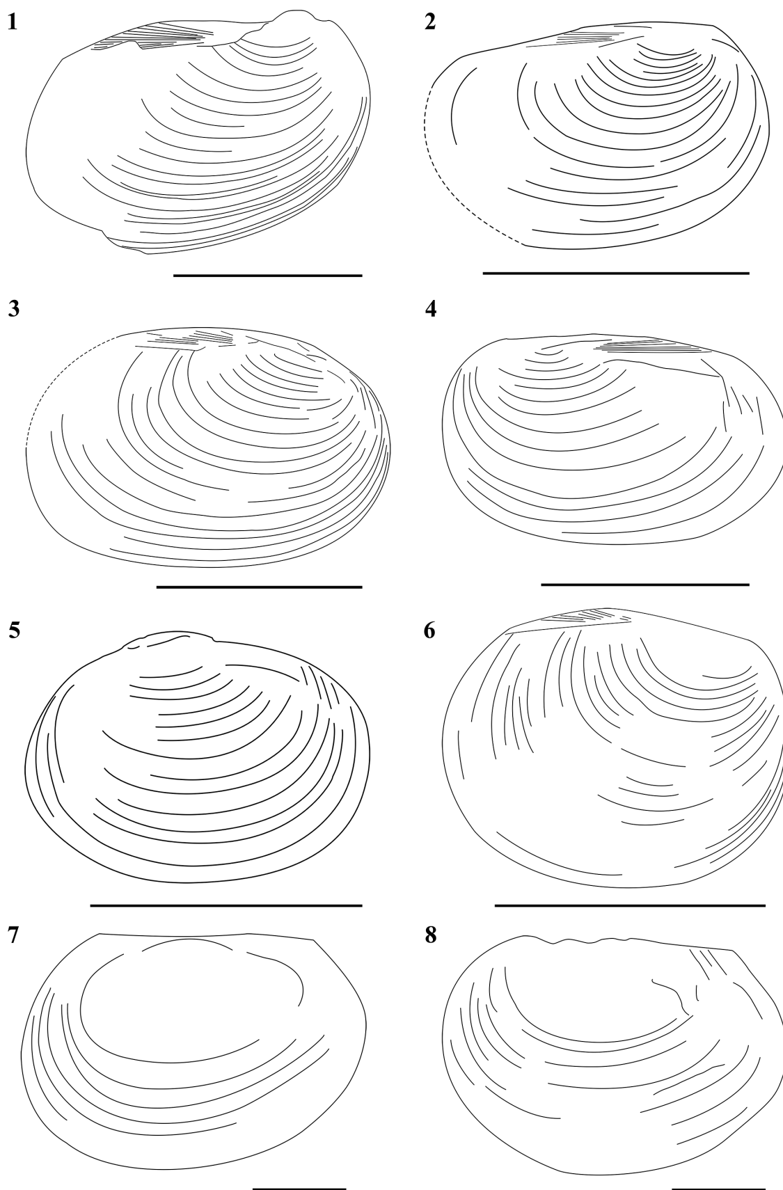
Figure 6. Line drawings of clam shrimp from Consthum. (1–6) Variation in Pseudestheria diensti . (1) Specimen EiB535a. (2) Specimen EiB551a_5. (3) Specimen EiB551b_1. (4) Specimen EiB559b. (5) Specimen EiB551b_7. (6) Specimen EiB552b_2. (7, 8) Palaeolimnadia stevenbeckeri n. sp. (7) Holotype EiB555. (8) Paratype EiB558. (1–6) Scale bars = 5 mm; (7, 8) scale bars = 1 mm.
