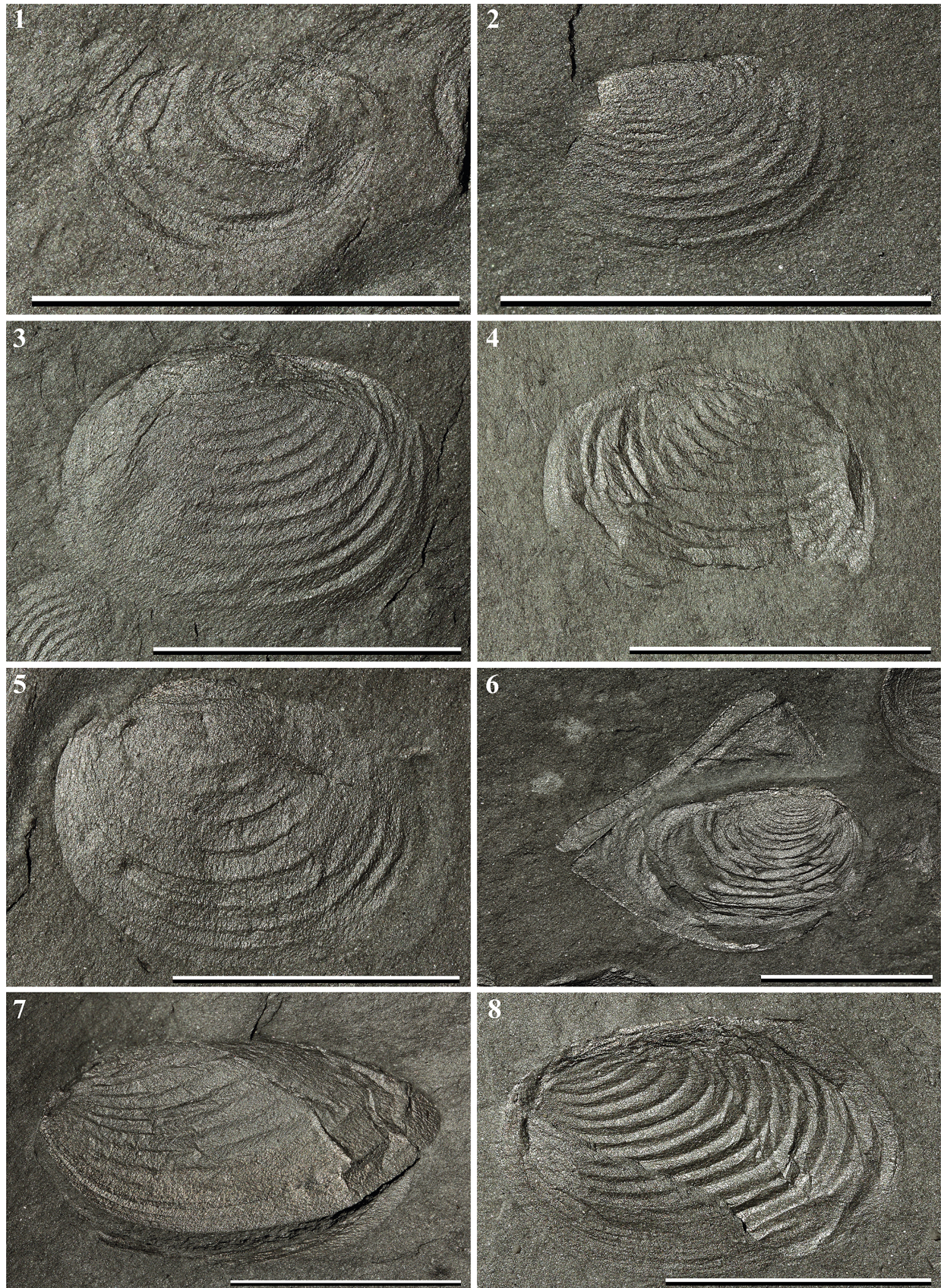
Figure 3. Individual clam shrimp specimens from the Consthum mass layer. (1) Undetermined, relatively small specimen EiB551b_3. (2) Undetermined, relatively small specimen EiB551b_4. (3) Pseudestheria diensti , mid-sized specimen, EiB551b_7. (4) Pseudestheria diensti , mid-sized specimen, EiB551b_5. (5) Pseudestheria diensti , EiB551b_2. (6) Pseudestheria diensti overlying Adelophthalmus sievertsi head shield, EiB551a_5. (7) Pseudestheria diensti , large specimen, EiB551b_10; note protruding right valve at lower margin. (8) Pseudestheria diensti , large specimen; note bivalved preservation. Scale bars = 5 mm.
