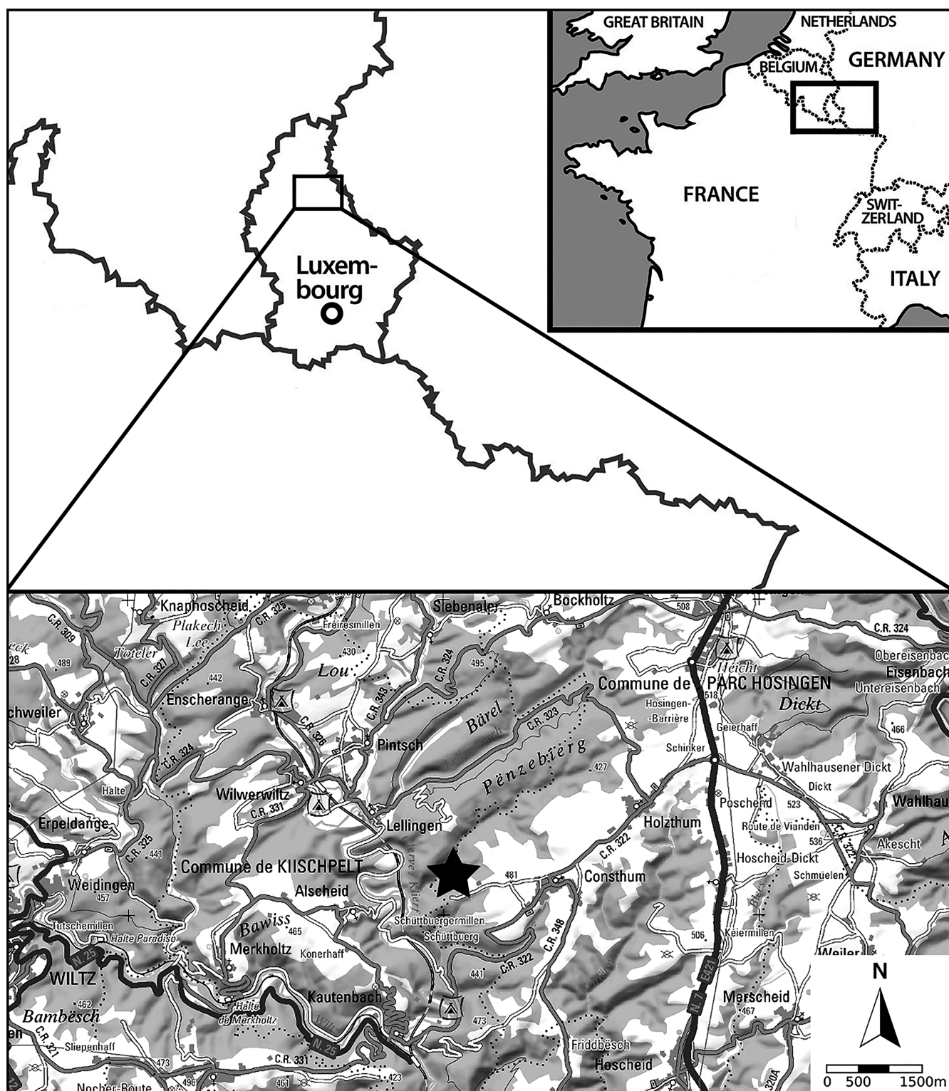
Figure 1. Geographical position of the Rinnen Quarry at Consthumb, Luxembourg.
