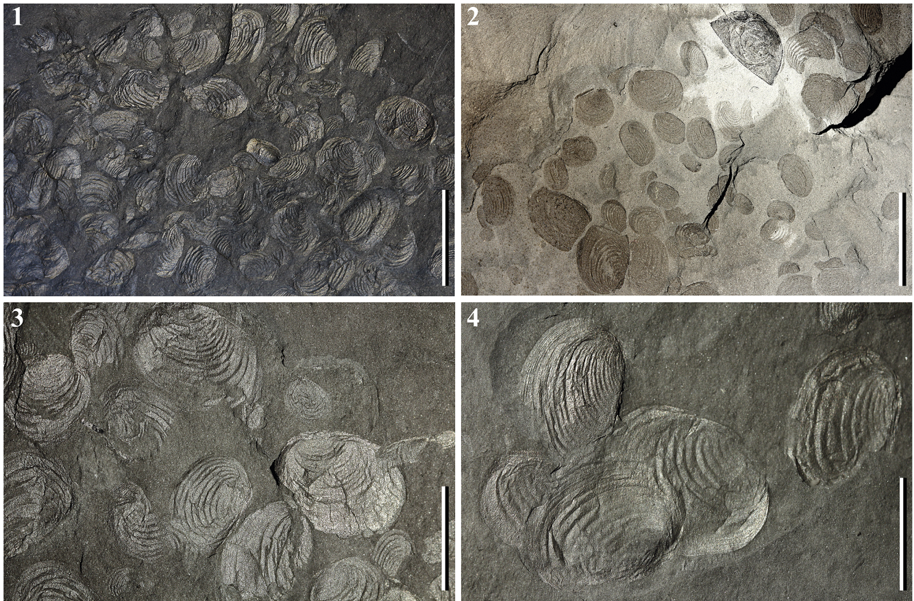
Figure 2. Examples from the Consthum clam shrimp mass layer. (1) Detail from slab EiB552b; note associated lingulid brachiopod near center. (2) Detail from slab EiB549a; note associated head shield of the eurypterid Adelophthalmus sievertsi (Störmer, 1969) (upper right), crossed polarizing filters. (3) Detail from slab EiB552a; note differences in size and form of dorsal margin. (4) Detail from slab EiB551a; note differences in the spacing of growth lines. (1, 2) Scale bars = 10 mm; (3, 4) scale bars = 5 mm.
