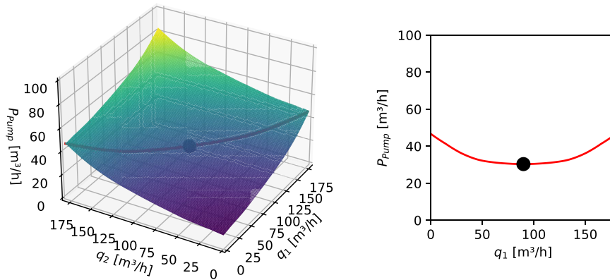
Figure 2. Example configuration consisting of two pumps. Left: An objective function dependent on two single pump flows q_1, q_2 with the cut line given by the pump station flow constraint (5) (red) and optimum. Right: The line to search (intersection of the objective function with the flow constraint [red line from left]) and the optimum.
