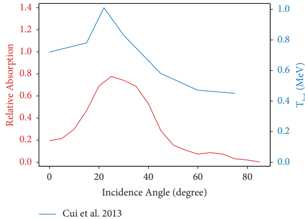
FIGURE 12: Plot of the absorption of energy in the Lorentz-boosted simulation in comparison to the data from Cui et al. [47].
