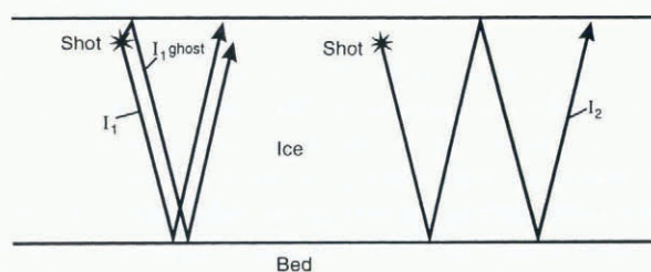
Fig. 3. Diagrammatic ray-paths for ice–bed reflection ( I_1 ), ice–bed ghost ( I_1 ghost) and first ice multiple ( I_2 ).
