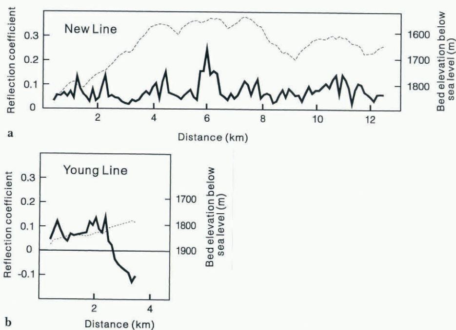
Fig. 8. Reflection coefficient (solid lines) of the ice-bed interface along (a) New Line and (b) Young Line. Dashed lines are the bed elevation profiles.
