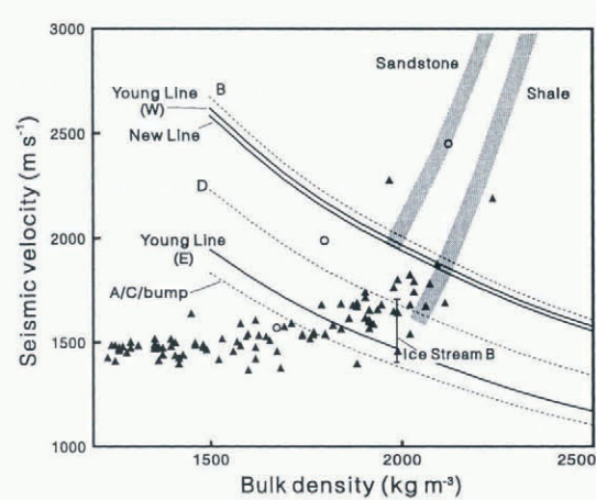
Fig. 10. Published values of density and seismic velocity for sediments and rocks, compared with lines of constant acoustic impedance determined for New Line and the various sections of Young and Tyree Lines. Modified from Smith (1997). Triangles are from saturated fresh-water sediments and from marine sediments, corrected to fresh-water values (following Blankenship and others, 1987b) where necessary. Sources are Nafe and Drake (1963), Morgan (1969) and Hamilton (1970). Open circles are from poorly lithified Cenozoic rocks from drillholes around McMurdo Sound, Ross Sea (Barrett and Froggatt, 1978). Vertical bar is the velocity and density for the bed of Ice Stream B (Blankenship and others, 1987b). Shaded areas show the lower ends of typical ranges for sedimentary rocks (e.g. Gardner and others, 1974).
