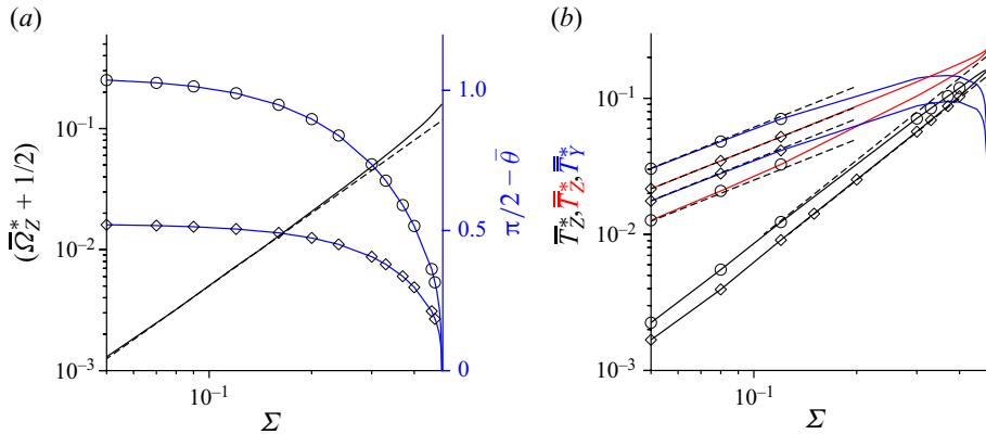
Figure 6. The variation in (a) (\bar{S}_Z^* + \frac{1}{2}) (black line) and \pi/2 - \bar{\theta} (blue line) and (b) \bar{T}_Z^* (black line), \bar{T}_Z^* (red line) and \bar{T}_Y^* (blue line) with the parameter \Sigma for \omega^* = 0.02 within the red rectangle in figure 4. The dashed black line in (a) is the \Sigma \ll 1 asymptotic solution (4.10). The dashed black lines in (b) are the \Sigma \ll 1 asymptotic solutions (4.12), (4.13) and (4.14). The initial conditions are \phi = 0 and \theta = (\pi/3) ( \circ ) and \theta = (\pi/6) ( \diamond ).
