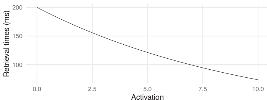
Figure 8. The retrieval time function.
