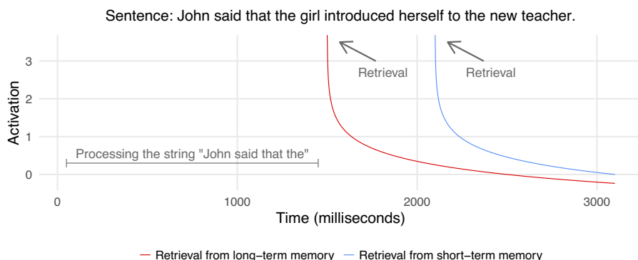
Figure 5. Fluctuation of the base-level activation of [ NP the girl] in (3) over time (see footnote 8). Two peaks correspond to retrievals at “girl” (from long-term memory) and “herself” (from short-term memory). Note: b = 0 , d = .5 .
