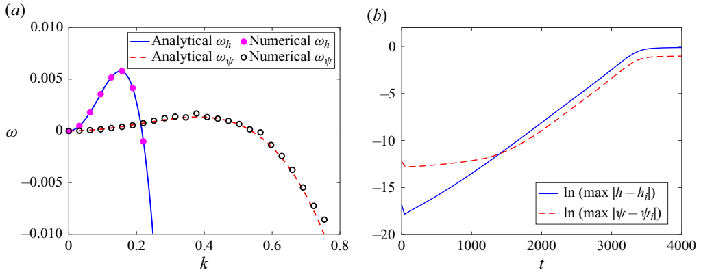
Figure 4. Results for a case with A' = 2 , K' = 0.15 , \alpha' = 1 , \epsilon' = 0.5 , a^2 = 2 , h_i = 2.2 and \phi_i = 0.4 . (a) Dispersion relation calculated numerically via (4.4) using \varepsilon_h = 10^{-7} , \varepsilon_\psi = 10^{-5} (symbols) compared with the analytic results in (3.10) and (3.11) (lines). (b) Measure of the evolution (cf. (4.5)).
