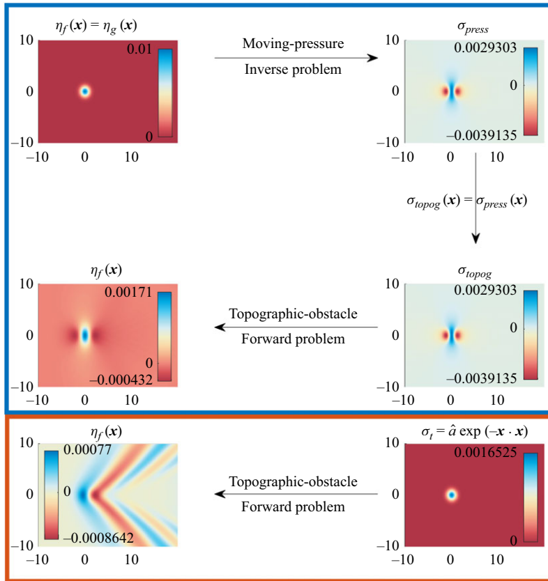
Figure 7. Fully nonlinear Euler system when Fr = 1.2 . Blue box: top left: \eta_f(x) for the moving-pressure distribution given by (4.9). Top right: the pressure-distribution, \sigma_{press}(x) that results in (4.9) when a = 0.01 . Middle right: the prescribed topographic-obstacle \sigma_{topog}(x) = \sigma_{press}(x) . Middle-left: the resulting free surface for \sigma_{topog}(x) . Red box: bottom right: Gaussian topographic obstacle with \hat{a} = 0.001653 chosen so it has identical mass to \sigma_{topog}(x) . Bottom left: free-surface response for the Gaussian topography.
