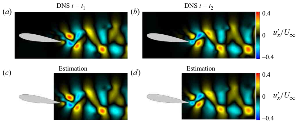
Figure 24. Estimation of the streamwise velocity fluctuation u'_x in an extended wake region for the nonlinear system with a clean free stream at two times: (a, b) DNS results, and (c, d) results from causal resolvent-based estimation.
